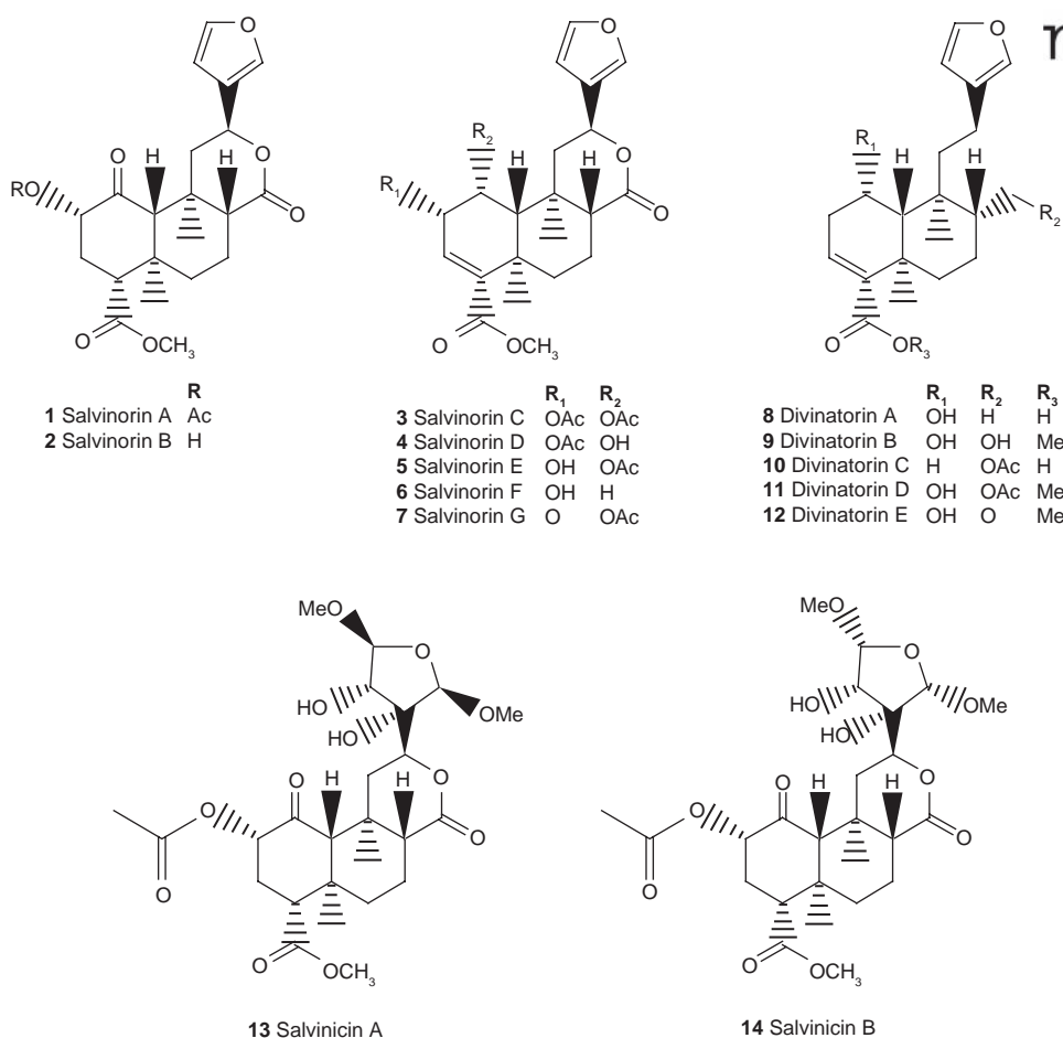
Figure 2. Structures of salvinorin A and B and related diterpenes isolated from Salvia divinorum .
