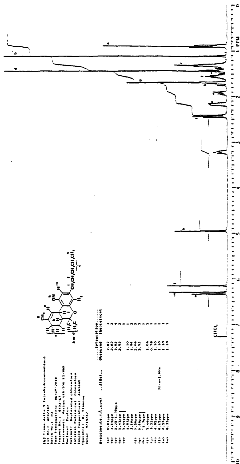
FIGURE 12 Nuclear Magnetic Resonance Spectrum of 1-Trans-Delta 9 -Tetrahydrocannabinol
