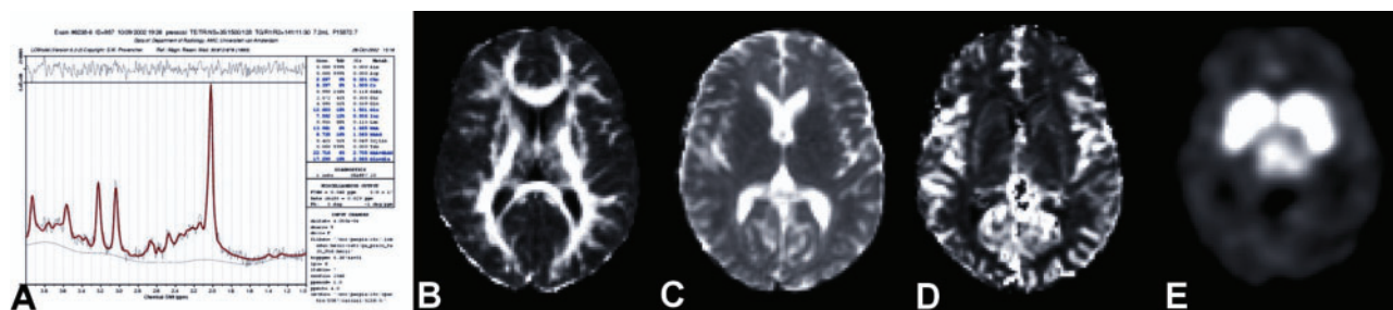
Fig. 1 Representative images of an individual (A) 1 H-MRS after analysis by LCModel and representative; (B) FA; (C) ADC; (D) rCBV and (E) [ 123 I]β-CIT binding images after transformation to the spatially normalized MNI brain template.
