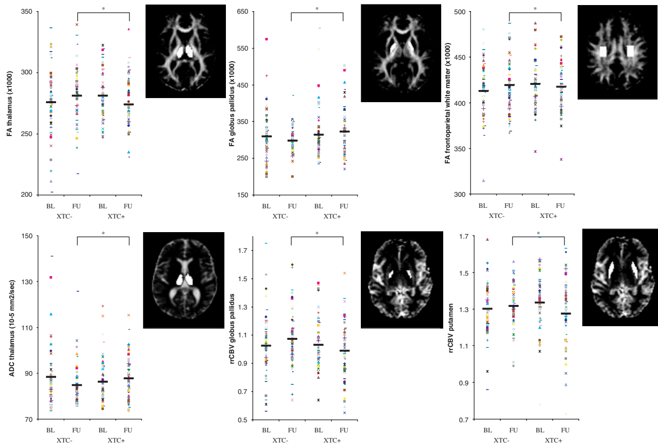
Fig. 2 Areas with significantly different findings between novel ecstasy users and persistent ecstasy-naïves at follow-up ( *P < 0.05 ), corrected for baseline measurements. Points represent individual and mean FA values in the thalamus, globus pallidus and frontoparietal white matter, ADC values in the thalamus and rCBV values in the globus pallidus and the putamen in ecstasy-naïves (XTC-) and novel ecstasy users (XTC+) at baseline (BL) and at follow-up (FU). In the right corner of each graph, the corresponding brain regions (marked in white) drawn on the FA, ADC and rCBV maps are given. Baseline scores were not significantly different between both groups ( P > 0.05 ). Only statistical significant results are shown, for complete results of all analyses see Table 2. Note that the vertical axis does not start at 0.
