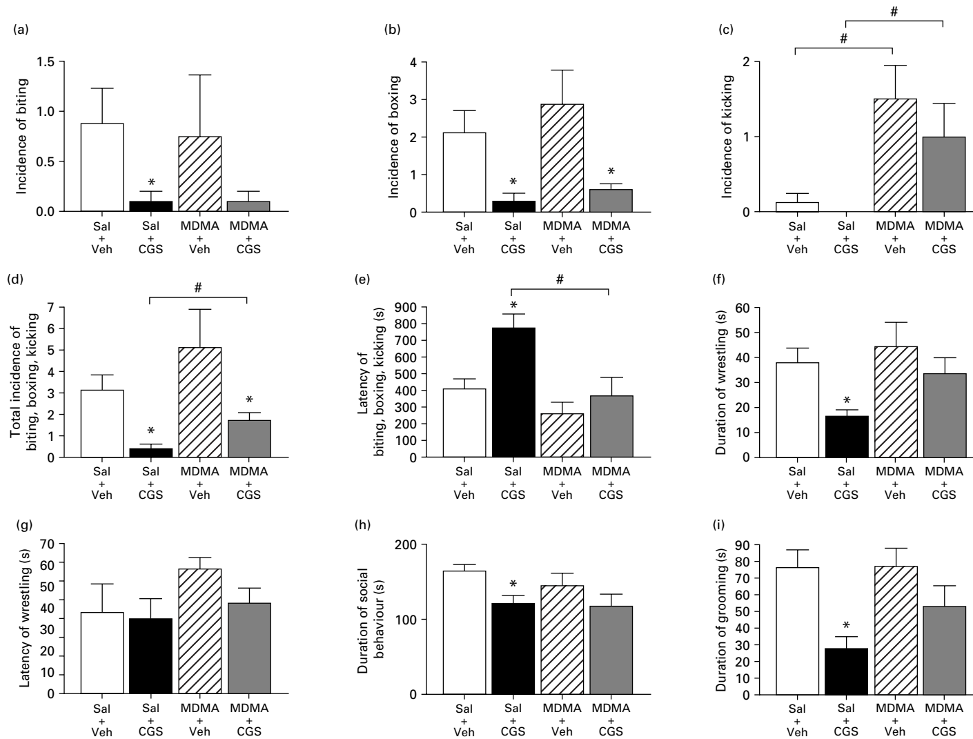
Figure 3. Acute effects of CGS-12066 (5 mg/kg) upon incidence of biting (a), boxing (b), kicking (c), total incidence (d) and latency (e) of biting, boxing, kicking, duration (f) and latency (g) of wrestling, duration of social behaviour (h) and grooming (i) in drug-naïve rats and in rats exposed to MDMA 3 wk earlier. Each group consisted of 6–10 animals [Sal + Sal ( n=8 ), Sal + CGS ( n=10 ), MDMA + Sal ( n=6 ), MDMA + CGS ( n=10 )]. * Significantly different from the appropriate control with the same pretreatment ( p < 0.05 ). # Significantly different from the saline-pretreated group with the same acute treatment ( p < 0.05 ). Sal, Saline; Veh, vehicle.
