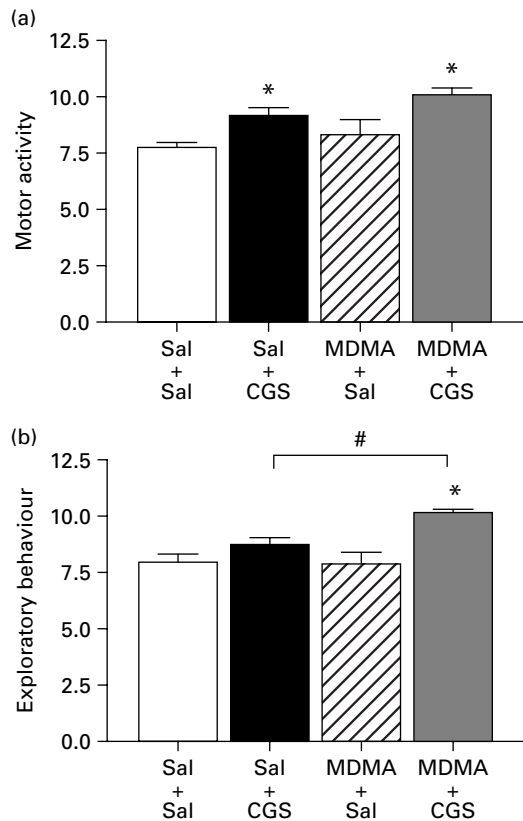
Figure 4. Acute effects of CGS-12066 (5 mg/kg) on motor activity and exploratory behaviour in drug-naïve rats and in rats exposed to MDMA 3 wk earlier. Each group consisted of 6–10 animals [Sal + Sal ( n=8 ), Sal + CGS ( n=10 ), MDMA + Sal ( n=6 ), MDMA + CGS ( n=10 )]. * Significantly different from the appropriate control with the same pretreatment ( p < 0.05 ). # Significantly different from the saline-pretreated group with the same acute treatment, ( p < 0.05 ). Sal, Saline.
