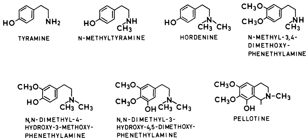
Fig. 1. Alkaloids identified in this study.
