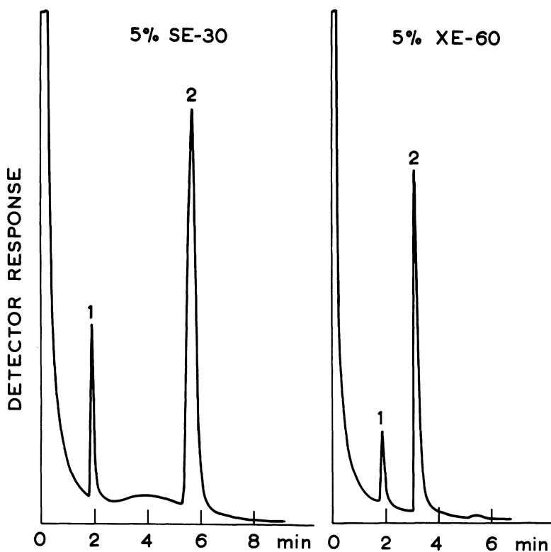
Fig. 4. Gas chromatograms of phenolic alkaloids of Pelecyphora aselliformis after preparative tlc in chloroform-ethanol-diethylamine (85:5:10). The fraction corresponding to hordenine (1) (above), was found also to contain an unknown compound (2), identified through mass spectrum and glc retention times as N,N-dimethyl-3-hydroxy-4,5-dimethoxyphenethylamine. Column temperature: 150°C.
