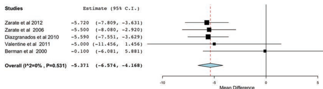
Figure 3. Forest plots for the efficacy of ketamine compared with placebo at baseline (top), 60–80 minutes (middle) and 210–230 minutes (bottom).
