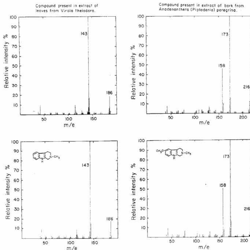
Fig. 6. Upper panel: mass spectra of "alkaloid 186" present in Viola theiodora and "alkaloid 216" present in Anadenanthera peregrina . Lower panel: mass spectra of reference compounds (IVa and IVb).
