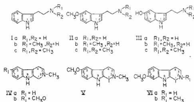
Fig. 1. Ia. tryptamine Ib. N -methyltryptamine Ic. N,N -dimethyltryptamine IIIa. 5-methoxytryptamine IIb. 5-methoxy- N -methyltryptamine IIc. 5-methoxy- N,N -dimethyltryptamine IIIa. 5-hydroxytryptamine (serotonin) IIIb. 5-hydroxy- N -methyltryptamine IIIc. 5-hydroxy- N,N -dimethyltryptamine (bufotenine) IVa. 2-methyltetrahydro- \beta -carboline IVb. 2-methyl-6-methoxytetrahydro- \beta -carboline V. 1,2-dimethyl-6-methoxytetrahydro- \beta -carboline VIa. tetrahydroharman VIb. 2-methyltetrahydroharman.
