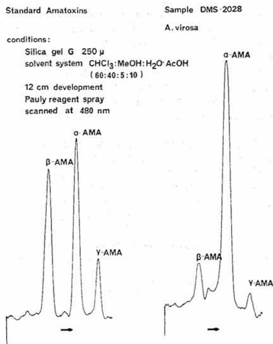
FIG. 1. Spectrodensitometric scan of the separation of amatoxins from Amanita virosa (DMS#2028); visualization reagent used was Pauly reagent, plate scanned at 480 nm.
