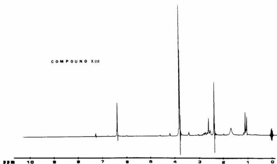
FIG. 25—NMR spectrum of 3,4,5-trimethoxy-N-methylamphetamine base in \text{CDCl}_3 .
