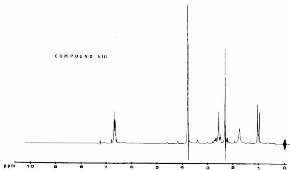
FIG. 20—NMR spectrum of 3,4-dimethoxy-N-methylamphetamine base in CDCl_3 .
