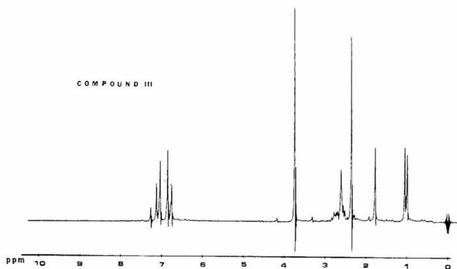
FIG. 15—NMR spectrum of 4-methoxy-N-methylamphetamine base in \text{CDCl}_3 .
