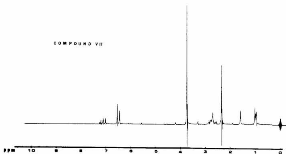
FIG. 19—NMR spectrum of 2,6-dimethoxy-N-methylamphetamine base in CDCl_3 .
