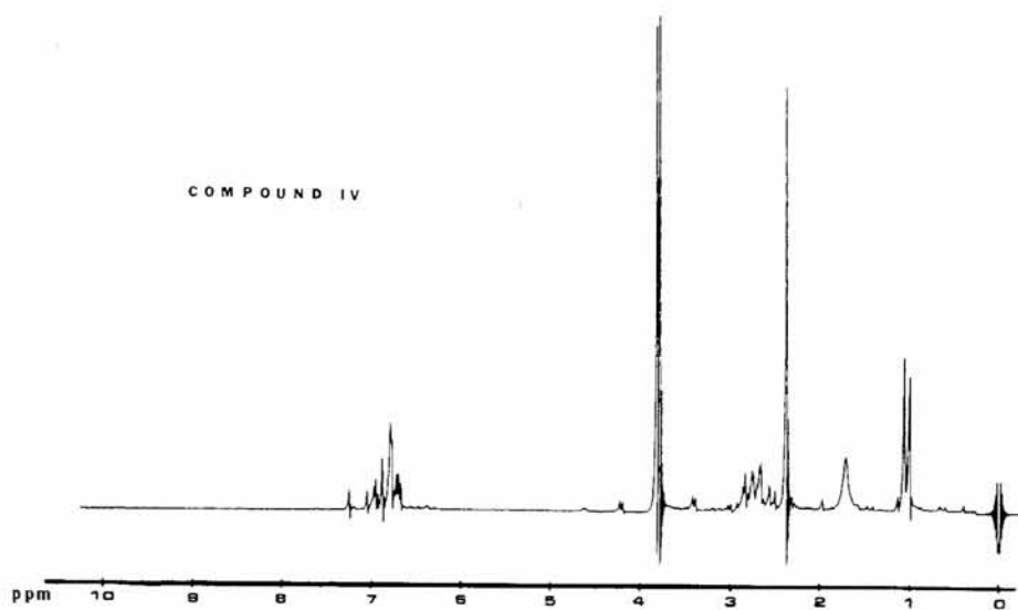
FIG. 16—NMR spectrum of 2,3-dimethoxy-N-methylamphetamine base in \text{CDCl}_3 .
