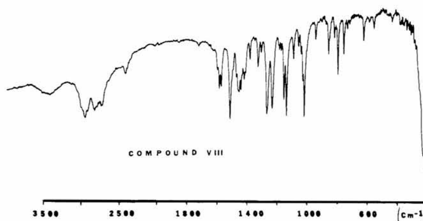
FIG. 7—IR spectrum of 3,4-dimethoxy-N-methylamphetamine HCl in KBr.
