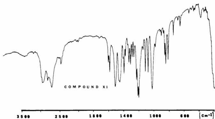
FIG. 10—IR spectrum of 2,4,5-trimethoxy-N-methylamphetamine HCl in KBr.
