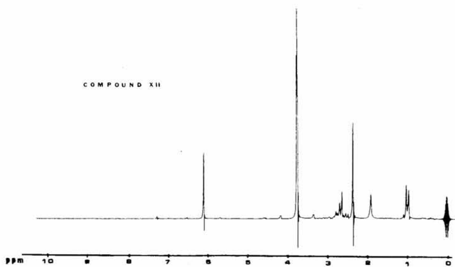
FIG. 24—NMR spectrum of 2,4,6-trimethoxy-N-methylamphetamine base in CDCl_3 .
