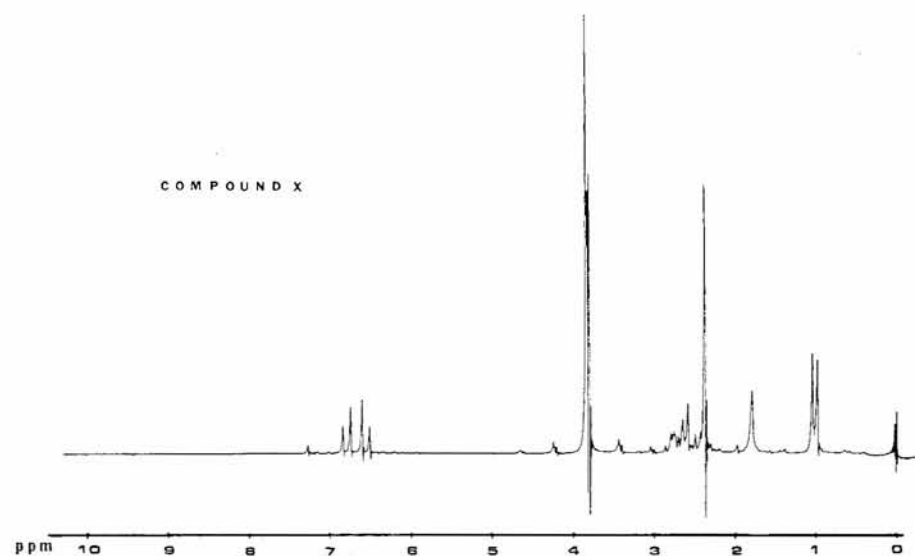
FIG. 22—NMR spectrum of 2,3,4-trimethoxy-N-methylamphetamine base in CDCl_3 .
