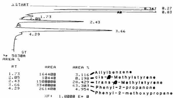
FIG. 18—Gas chromatogram of the allylbenzene modified procedure after 19 h.
