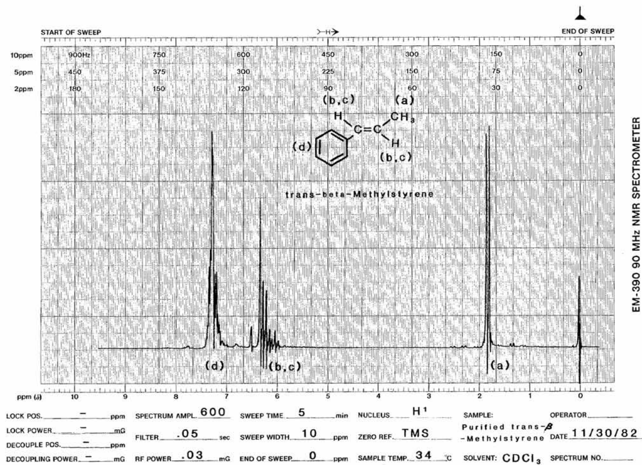
FIG. 12—Nuclear magnetic resonance spectrum ( CDCl_3 ) for trans-beta-methylstyrene.
