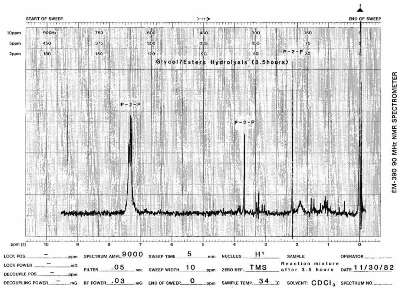
FIG. 28—Nuclear magnetic resonance spectrum of trans - \beta -methylstyrene hydrolysis after 3\frac{1}{2} h.
