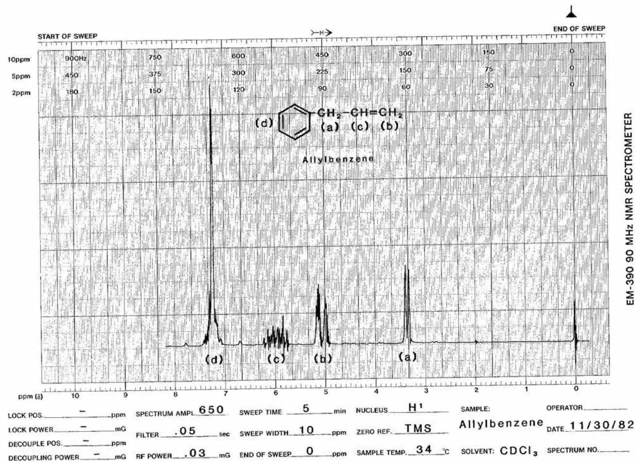
FIG. 11—Nuclear magnetic resonance spectrum (CDCl 3 ) for allylbenzene.
