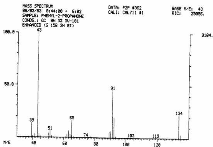
FIG. 10—Mass spectrum for phenyl-2-propanone.
