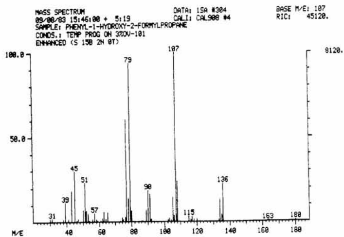
FIG. 24—Mass spectrum of phenyl-1-hydroxy-2-formyl-propane.
