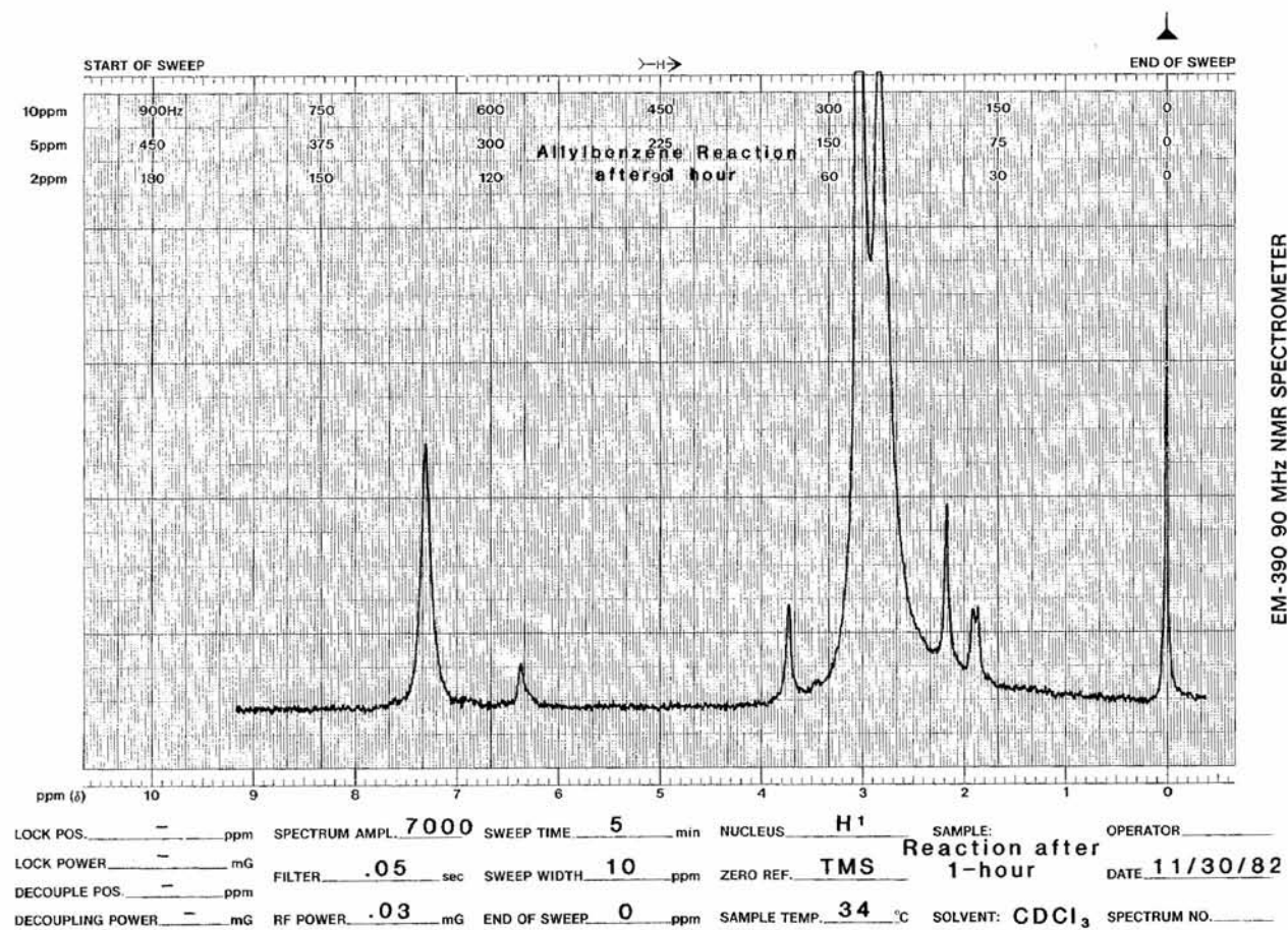
FIG. 14—Nuclear magnetic resonance spectrum of allylbenzene reaction mixtures—literature procedure after 1 h.
