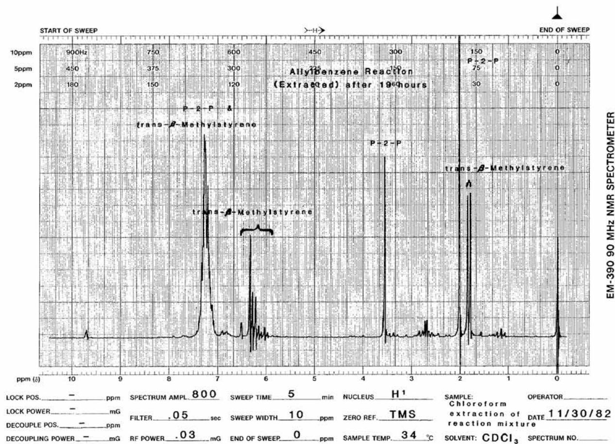
FIG. 19—Nuclear magnetic resonance spectrum of allylbenzene reaction mixtures—literature procedure after 19 h (extracted).
