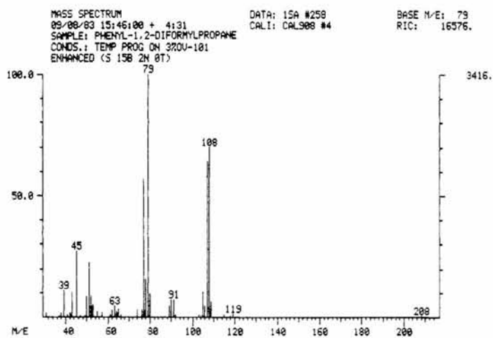
FIG. 26—Mass spectrum of phenyl-1,2-diformyl propane.
