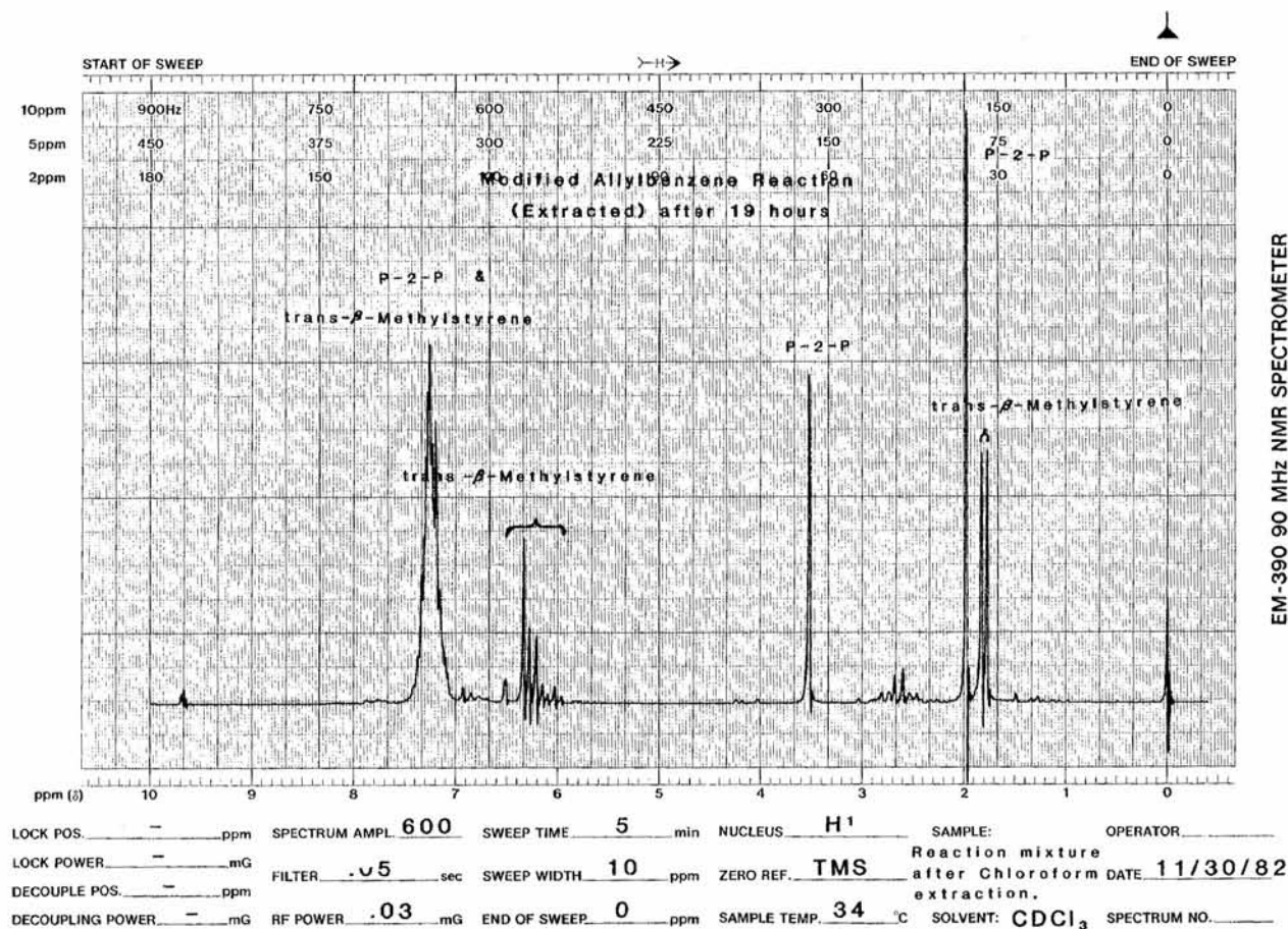
FIG. 20—Nuclear magnetic resonance spectrum of allylbenzene reaction mixtures—modified procedure after 19 h (extracted).
