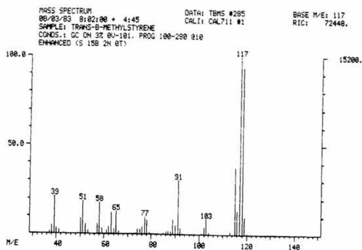
FIG. 9—Mass spectrum for trans-beta-methylstyrene.
