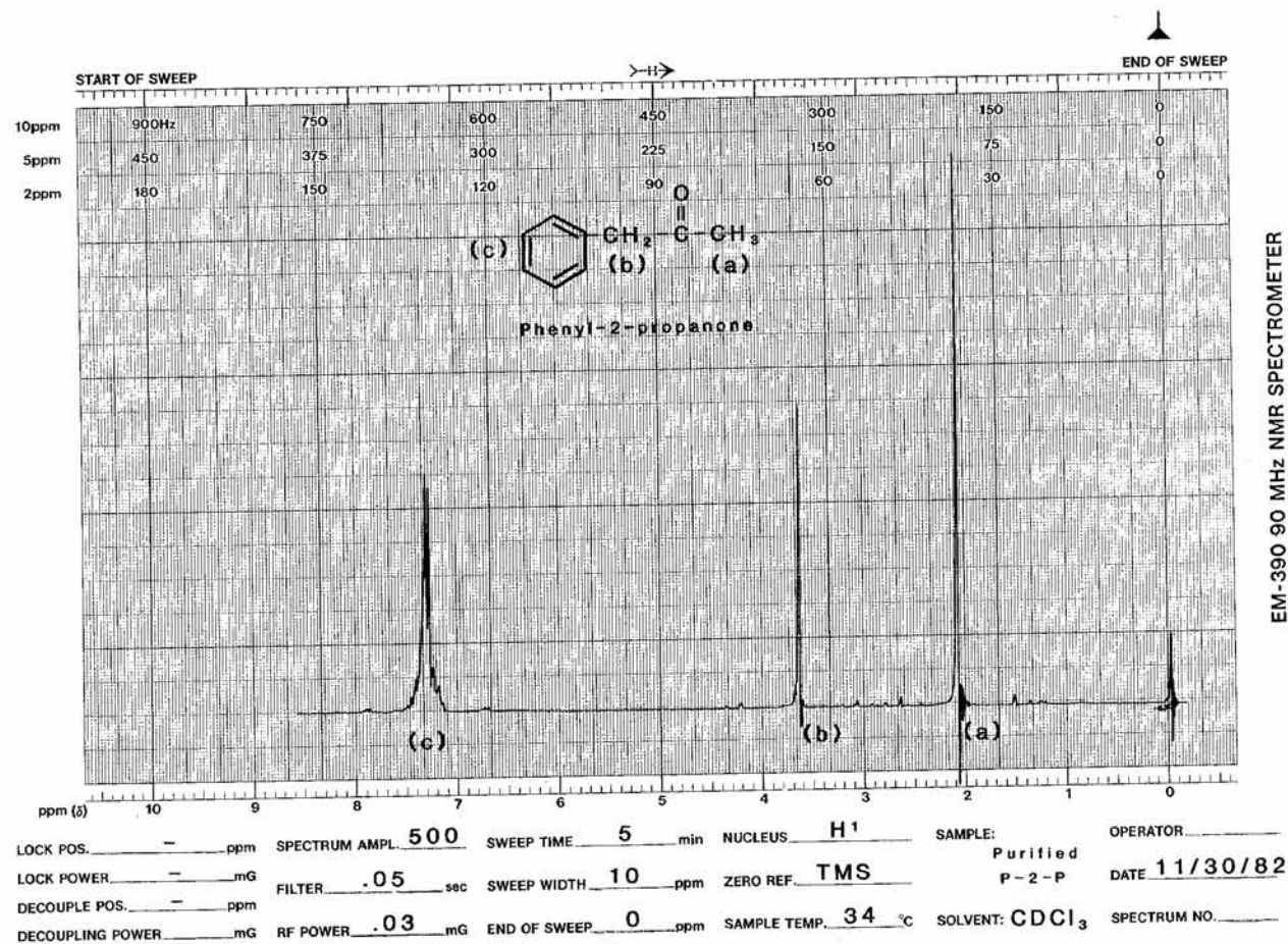
FIG. 13—Nuclear magnetic resonance spectrum ( CDCl_3 ) for phenyl-2-propanone.
