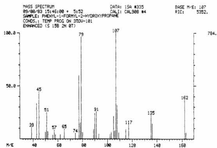
FIG. 25—Mass spectrum of phenyl-1-formyl-2-hydroxypropane.
