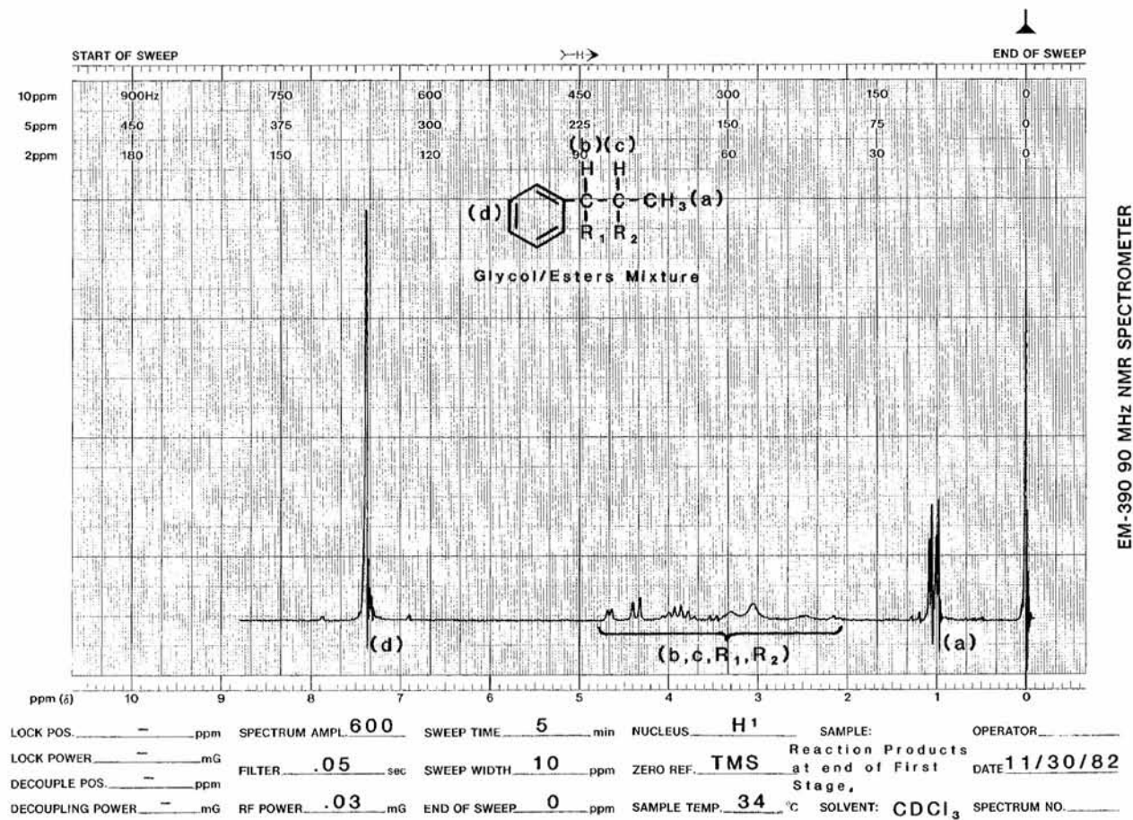
FIG. 22—Nuclear magnetic resonance spectrum of the trans-beta-methylstyrene oxidation mixture.
