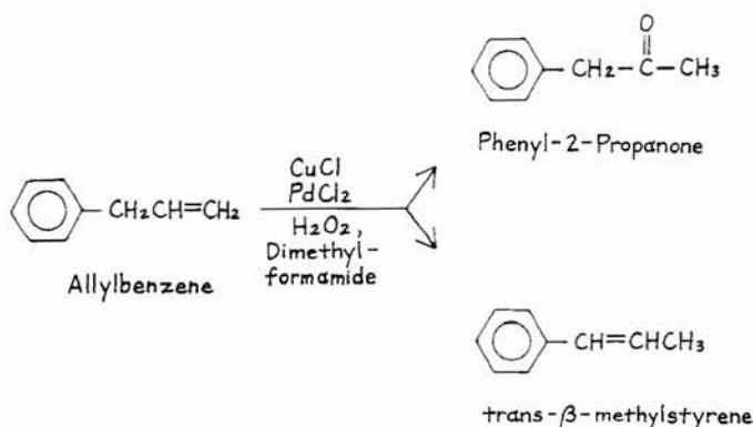
FIG. 2—Synthetic procedure for phenyl-2-propanone—modified allylbenzene method.
