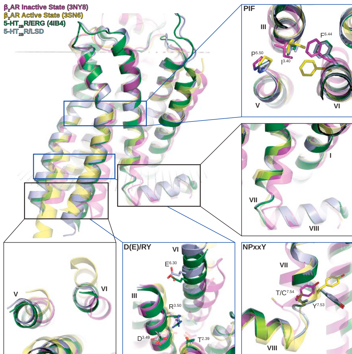
Figure S2. Activation States of 5-HT 2B R/LSD and 5-HT 2B R/ERG through Comparison with the \beta_2 Adrenergic Receptor, Related to Figure 2 Superposition of 5-HT 2B R/LSD (light blue), 5-HT 2B R/ERG (dark green) (PDB ID: 4IB4 (Wacker et al., 2013)), \beta_2 AR/ICI 118,551 (transparent magenta) (PDB ID: 3NY8 (Wacker et al., 2010)), and the \beta_2 AR-Gs complex (transparent yellow) (PDB ID: 3SN6 (Rasmussen et al., 2011b)) aligned through helices I-IV. Close ups highlight activation related changes in the PIF, D(E)/RY, and NPxxY motifs, as well as activation related movements in the cytoplasmic portions of helix V, VI, and VII. For better illustration of a cytoplasmic view of helix V, VI, and D(E)/RY, as well as an extracellular view of the PIF motif, parts of the receptors were removed. Membrane boundaries are indicated by gray dots according to the Orientations of Proteins in Membranes database (Lomize et al., 2006).
