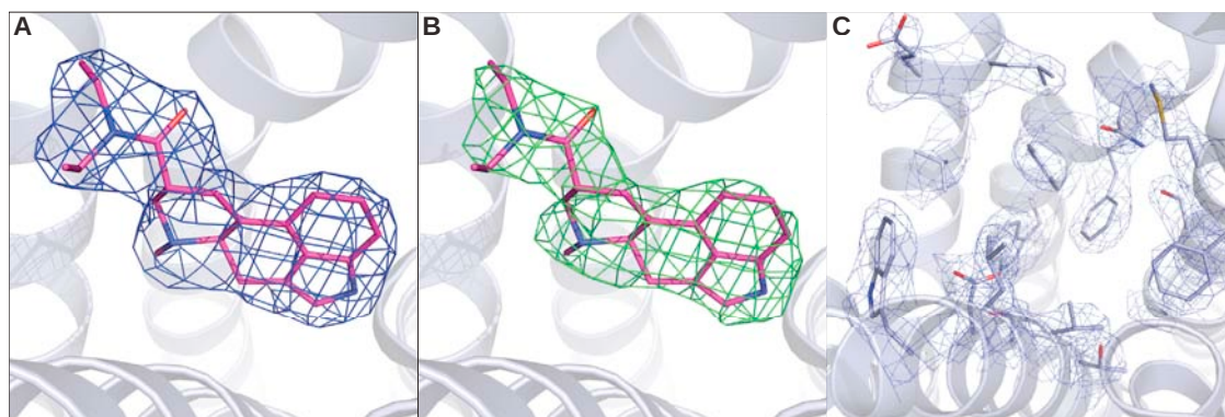
Figure S1. Electron Density of LSD and Ligand Binding Pocket Residues, Related to Figure 1
