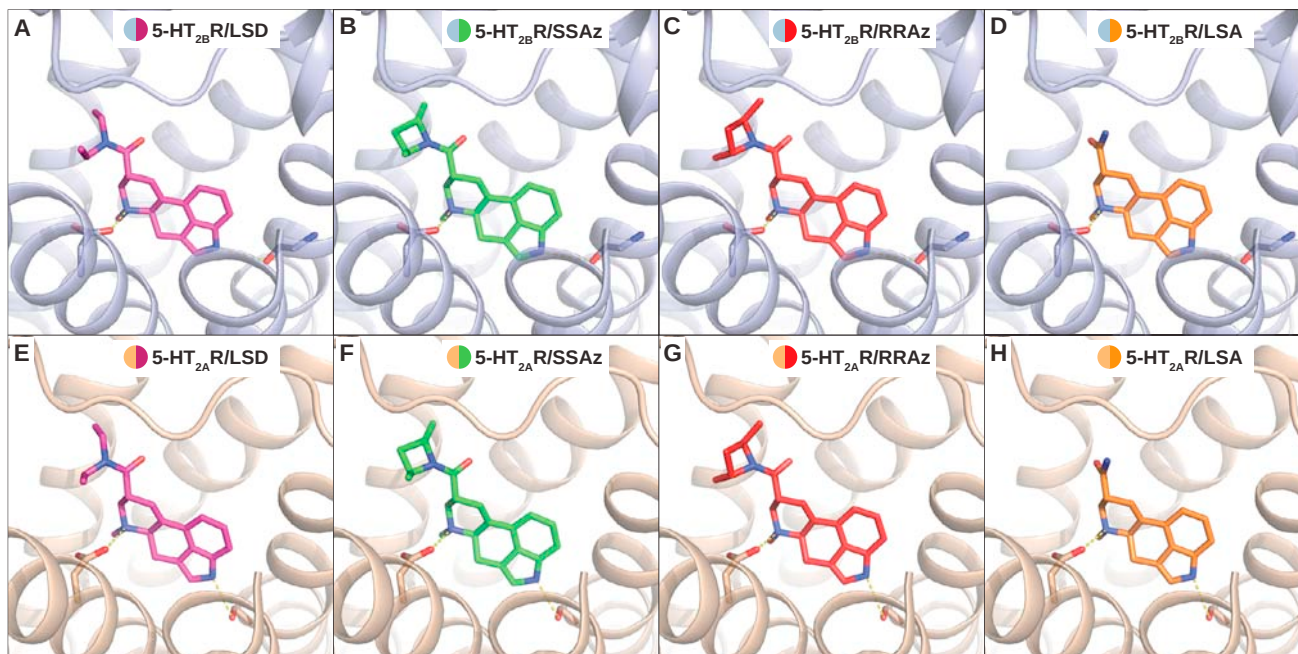
Figure S4. Docking of LSD Derivatives into 5-HT 2B R Structure and 5-HT 2A R Homology Model, Related to Figure 3
