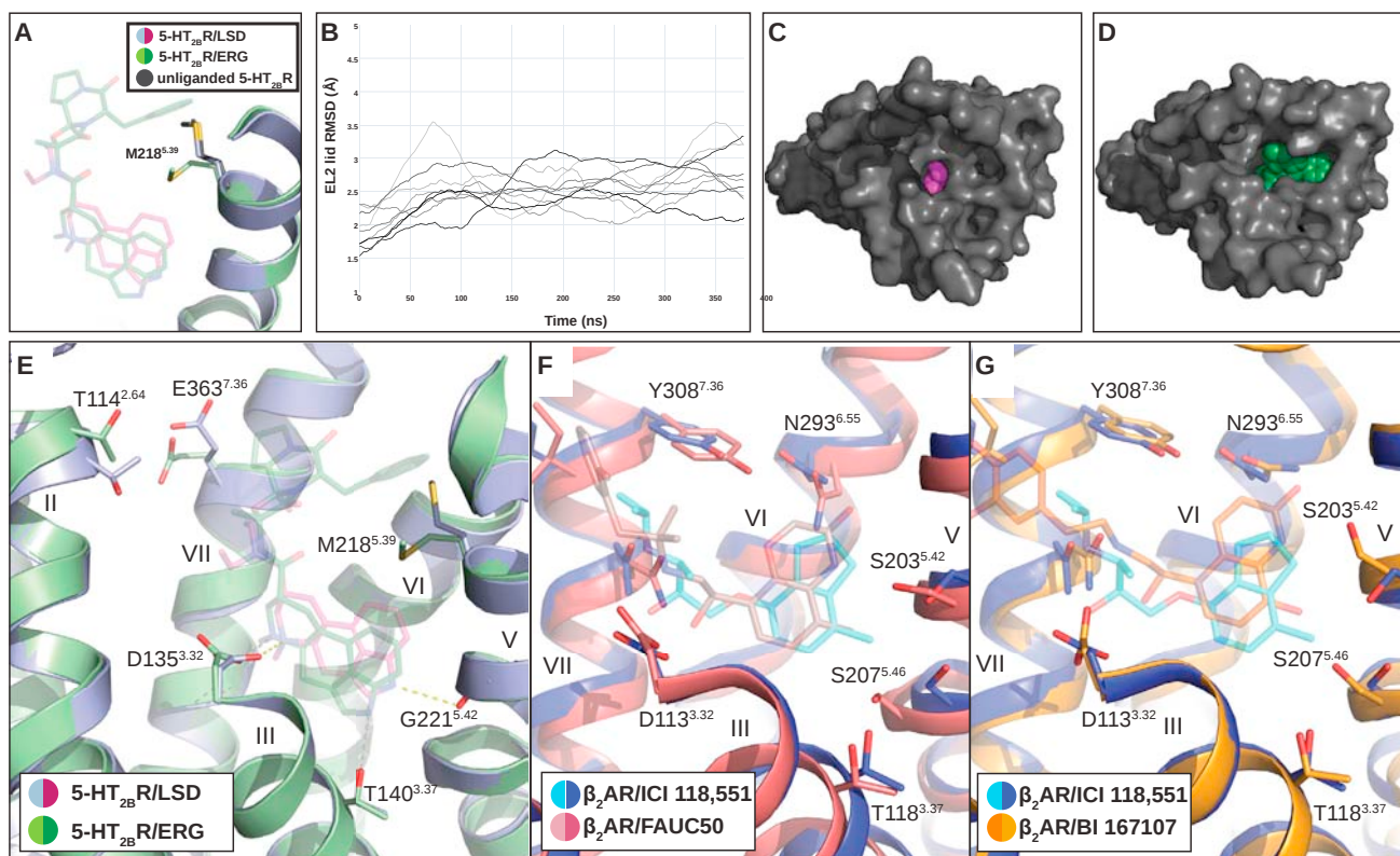
Figure S3. MD Simulations of 5-HT 2B R Complexes, Differences in LSD versus Ergotamine Surfaces, and Conformational Changes between 5-HT 2B R/LSD and 5-HT 2B R/ERG Binding Pockets Compared with Activation-Related Changes Observed in the \beta_2 AR Binding Pocket, Related to Figures 2 and 4
