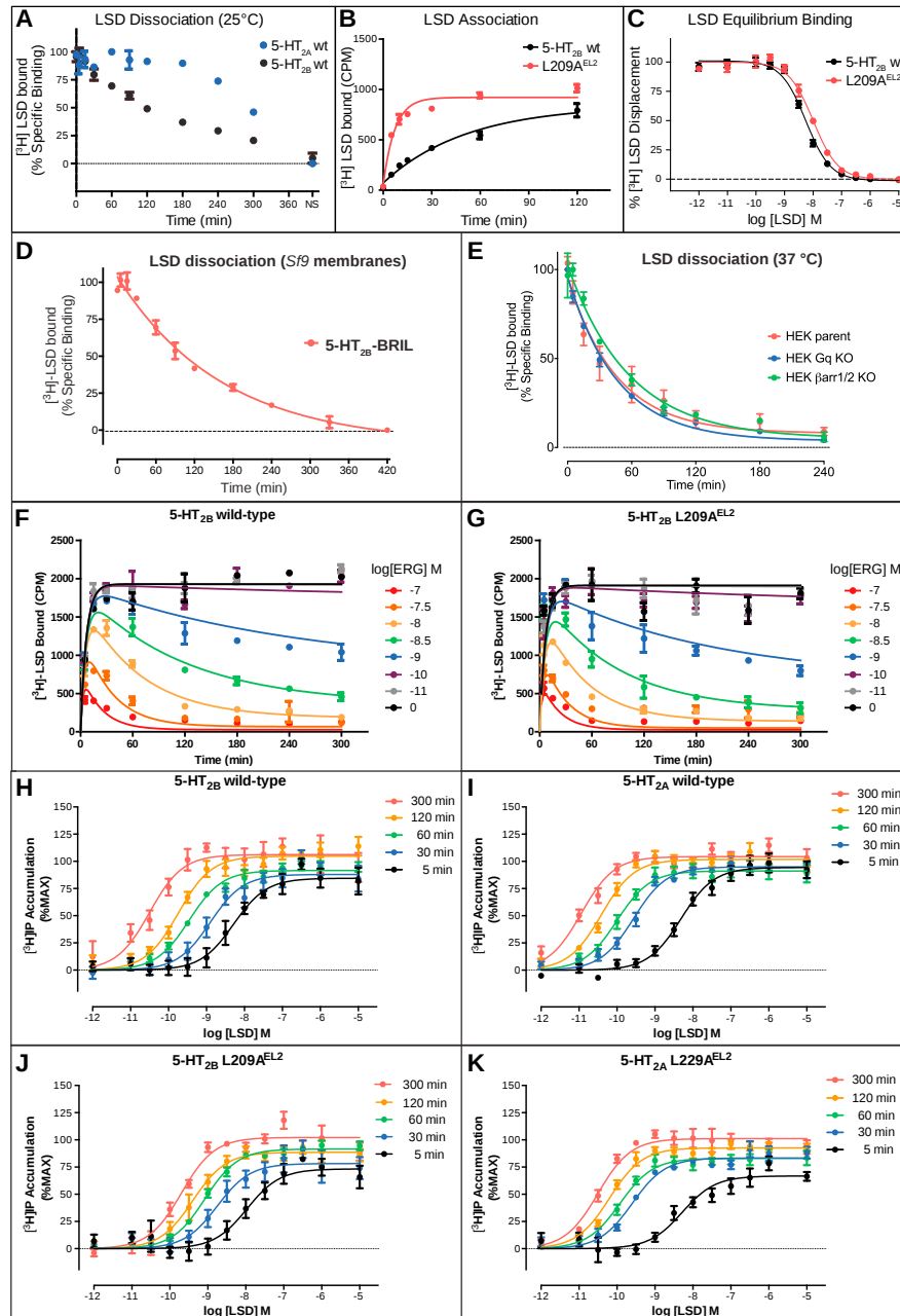
Figure S5. LSD Binding and Signaling Kinetics, Related to Figures 4 and 5
