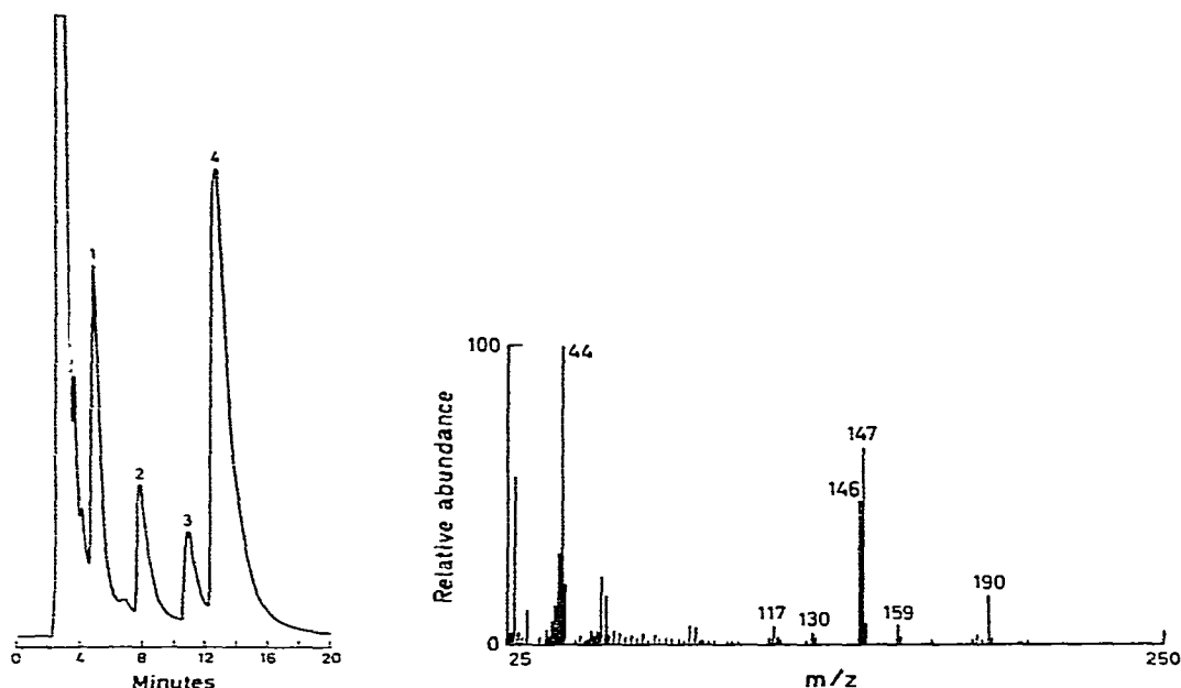
Fig. 1. HPLC chromatogram of a methanolic extract of Norwegian P. semilanceata . Peaks: 1, 2 = unknown; 3 = baeocystin; 4 = psilocybin. Mobile phase: methanol-water-1 M ammonium acetate, pH 9.6 (240:50:10); flow-rate, 1 ml/min. Detector wavelength: 254 nm. Injected volume: 100 \mu l.
