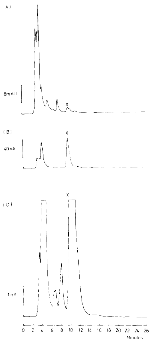
Fig. 3. Chromatograms of Panaeolus rickenii after (A) UV detection; (B) fluorescence detection; (C) electrochemical detection. Detector characteristics as in Fig. 2. Peak X = unknown.
