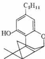
Cannabicyclol (CROMBIE et al., 1968)
