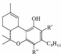
\Delta^1 -THC acid A R' = \text{COOH}, R'' = \text{H} (KORTE et al., 1965) \Delta^1 -THC acid B R' = \text{H}, R'' = \text{COOH} (MECHOUAM et al., 1969)
