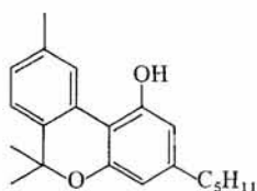
Cannabinol (CBN) (ADAMS et al., 1940)
