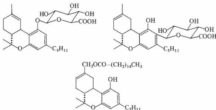
Fig. 6. Examples of phase II cannabinoid metabolites
