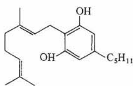
Cannabigerol (GAONI and MECBOULAM, 1964b)
