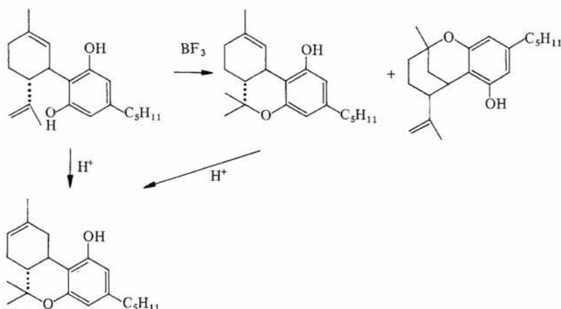
Fig. 2. Some transformations of cannabinoids in acids
