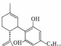
Cannabidiol (CBD) (MECHOUAM and SHVO, 1963)
