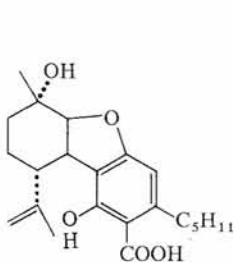
Cannabielsoic acid A (SHANI and MECBOULAM, 1974)
