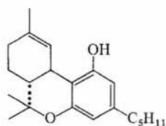
\Delta^1 -Tetrahydrocannabinol ( \Delta^1 -THC, also named \Delta^9 -THC) (GAONI and MECBOULAM, 1964a)
