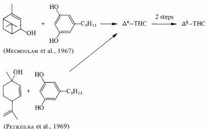
Fig. 3. Some syntheses of \Delta^1 -THC
