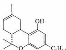
\Delta^6 -THC (also named \Delta^8 -THC) (HIVELY et al., 1966)
