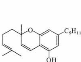
Cannabichromene (CLAUSSEN et al., 1966; GAONI and MECBOULAM, 1966)
