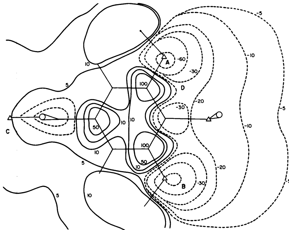
FIG. 4. IV. Approximate electrostatic potential for 3,5-dimethoxy-4-methylthiophenethylamine in kcal/mol
