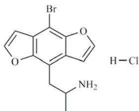
Fig. (1). 1-(8-bromobenzo[1,2- b :4,5- b' ]difuran-4-yl)-2-aminopropane hydrochloride (Bromo-Dragonfly).
