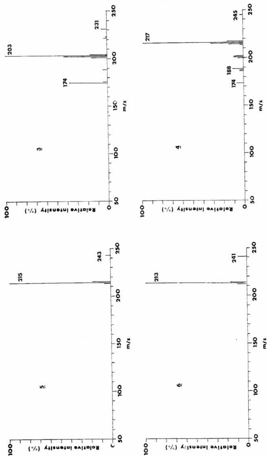
Fig. 5. The CI mass spectra of compounds 3-6.
