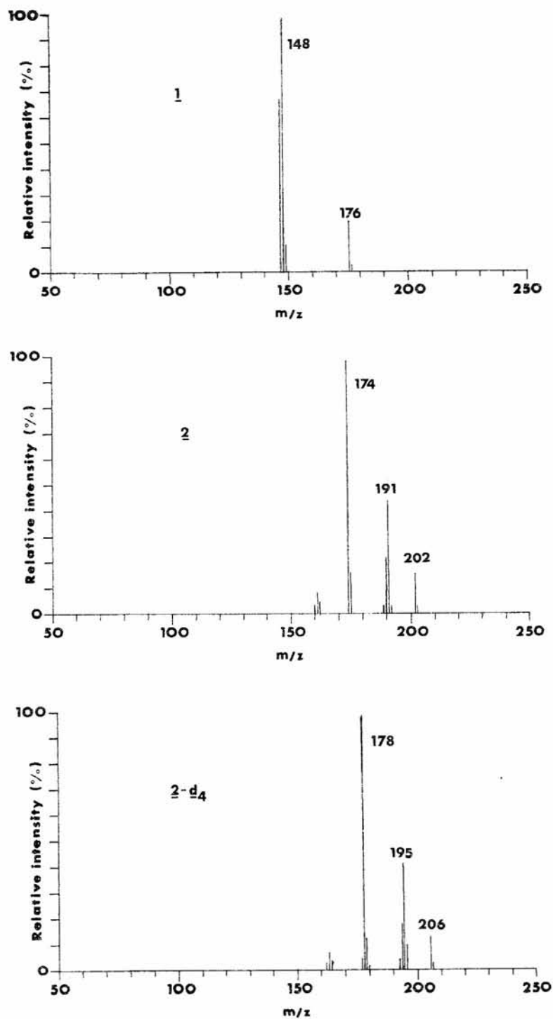
Fig. 3. The CI mass spectra of compounds 1, 2 and 2-d 4 .
