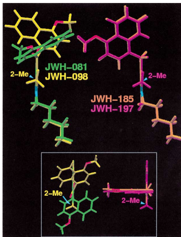
Figure 1. (Left) A side view is shown here in which the global minimum energy conformers of JWH-081 ( 16 , s-trans ; in green) and JWH-098 ( 19 , s-cis ; in yellow) are superimposed at their indole rings. In this side view, the indole ring is perpendicular to the page with the 2-methyl group pointing towards the viewer. In the cutout at the bottom, molecules are oriented in a top view, so that the indole ring is perpendicular to the page with C-4 pointing towards the viewer and the C-2 methyl of 19 pointing down. The alkyl side chains have been removed here in order to simplify the display. (Right) A side view is shown here in which the global minimum energy conformers of JWH-185 ( 11 , in orange) and JWH-197 ( 14 , in purple) are superimposed at their indole rings. In this side view, the indole ring is perpendicular to the page with the 2-methyl group pointing towards the viewer. In the cutout at the bottom, molecules are oriented in a top view so that the indole ring is perpendicular to the page with C-4 pointing towards the viewer and the C-2 methyl of 19 pointing down. The alkyl side chains have been removed here in order to simplify the display.
