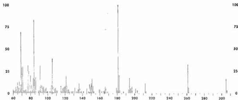
Fig. 1—Mass spectrum of peyonine.
