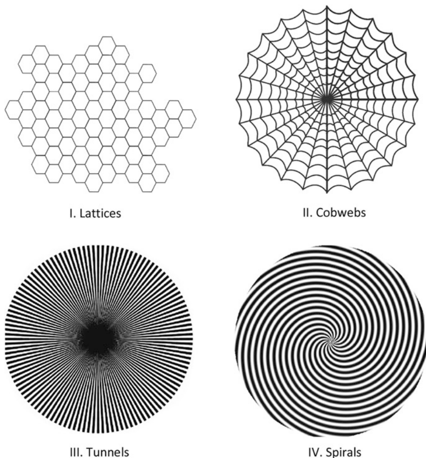
Fig. 1 Sample stimuli for the four hallucinatory form constants: (I) lattices (including gratings, fretworks, honeycombs, filigrees, and chessboard designs), (II) cobwebs, (III) tunnels (including alleys, funnels, cones, and vessels) and (IV) spirals.
