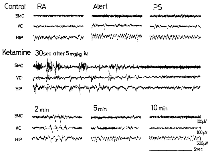
FIG. 1. Effects of intravenously-administered ketamine on the electroencephalographic pattern of an unrestrained cat. SMC, sensorimotor cortex; VC, visual cortex; Hip, hippocampus. Top, records made during arousal at rest (RA), alertness (Alert) and paradoxical sleep (PS). Center, from 30 to 50 sec after ketamine, 5 mg/kg, was injected. The cat was asleep (slow-wave sleep). Toward the right the EEG's were all desynchronized. Bottom, records made 2, 5, and 10 min after injection. EEG seizures are evident at 2 min. The VC record at 5 min still shows EEG seizures.
