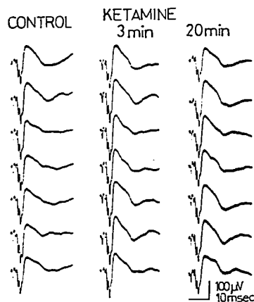
FIG. 5. Enhancement of sensorimotor cortical evoked potentials by ketamine. Single shocks were applied to the medial lemniscus. Control records were obtained during arousal at rest. Sweeps in each column were consecutive.
