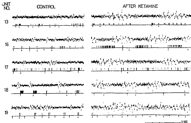
FIG. 9. Effects of ketamine on unitary activity of the visual cortex. Left, control records obtained during arousal at rest. Right, 1-3 min after injection of ketamine, 2 mg/kg. In each row the upper record is the background EEG and the lower one, unitary spikes shaped by a Schmitt circuit. Arrows below the unitary spikes indicate stimulation by a moving shadow. Changing directions of the arrows mean that the direction of the shadow was changed (see text).
