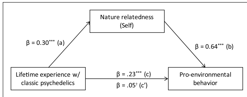
Figure 2. Mediation analysis. \beta s represent standardized regression coefficients. (c) indicates the total effect, (c') indicates the direct effect when controlling for the indirect effect ( a \times b ). Other variables in the structural equation model are not displayed, but statistically accounted for.
