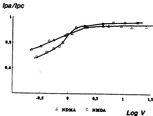
FIGURE 4. Dependence of the I_{pa}/I_{pc} ratio with the sweep rate for the nitroamphetamine derivatives.
