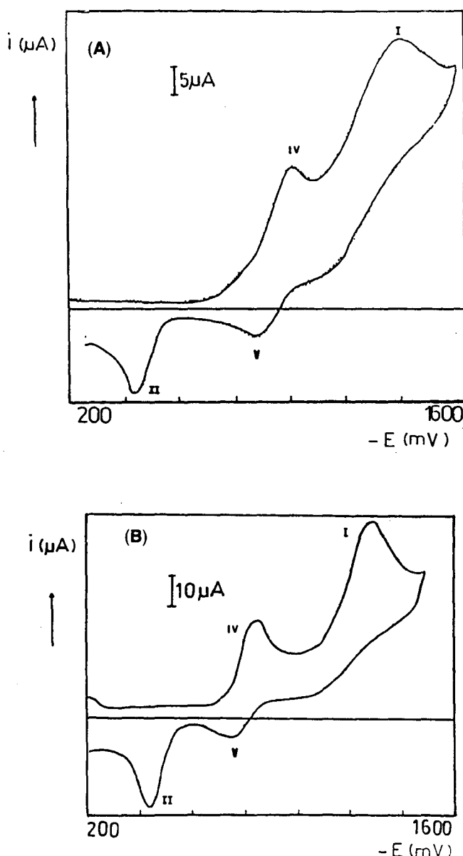
FIGURE 2. Cyclic voltammograms of the nitroamphetamine derivatives in the optimal mixed media conditions at 1 mM concentration. (A) NDMA in aqueous citrate buffer pH 10/DMF [50/50]. (B) NMDA in aqueous citrate buffer pH 10.5/DMF [30/70].
