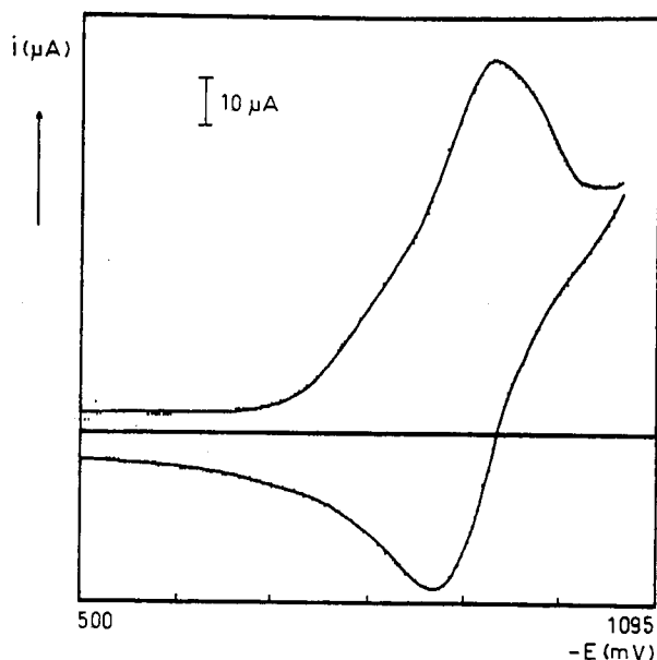
FIGURE 3. Cyclic voltammogram for the isolated \text{Ar-NO}_2/\text{Ar-NO}_2^- couple of NMDA, in aqueous citrate buffer pH 10.5/DMF [30/70].
