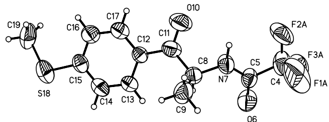
Figure 3. ORTEP projection of 1c .
