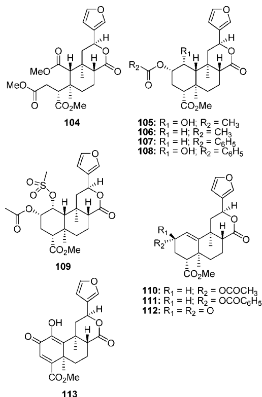
Figure 8. Ring A modified salvinorin A analogs.
