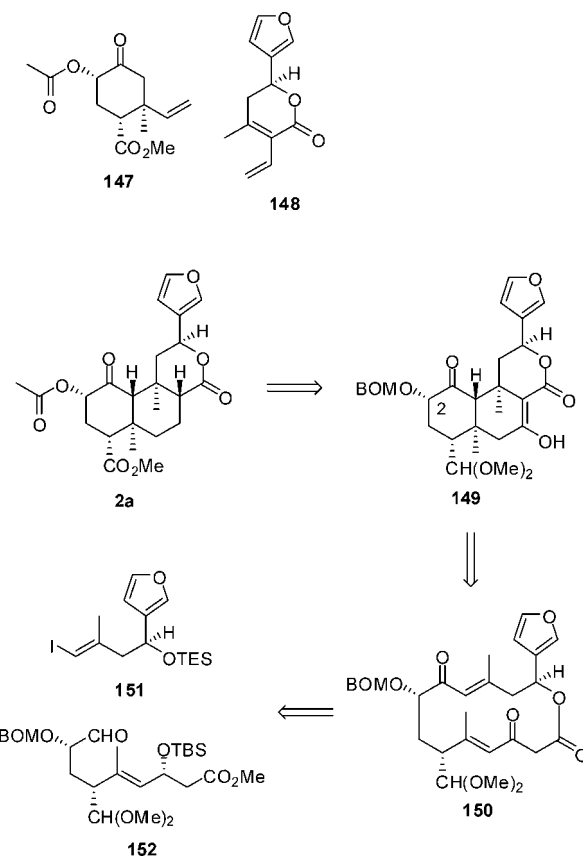
Figure 12. Synthetic targets and intermediates used in synthesis efforts of salvinorin A. Adapted from ref 91.
