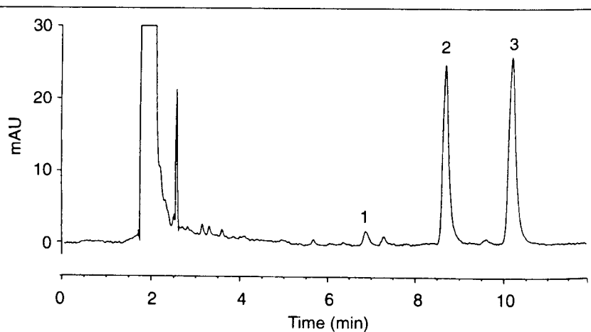
Figure 2. HPLC profile of a plasma extract; subject B, 120 min after an oral dose of 1.5 mg/kg 3,4-methylenedioxymethamphetamine (MDMA). Peaks: 1, 3,4-methylenedioxyamphetamine (MDA, 3.9 ng/mL); 2, methamphetamine (MA, internal standard); 3, 3,4-methylenedioxymethamphetamine (MDMA, 331.3 ng/mL).
