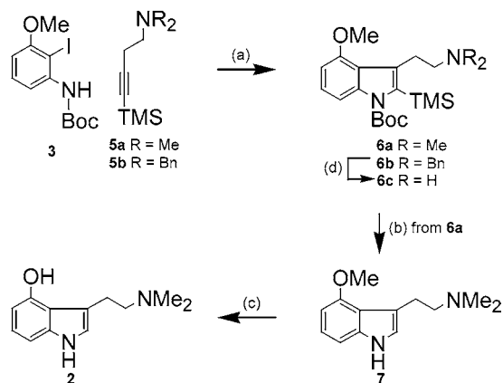
Scheme 2. Synthesis of Psilocin a
