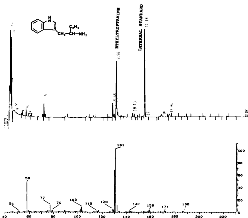
FIG. 2—Structural formula, total ion chromatogram and mass spectra of etryptamine.
