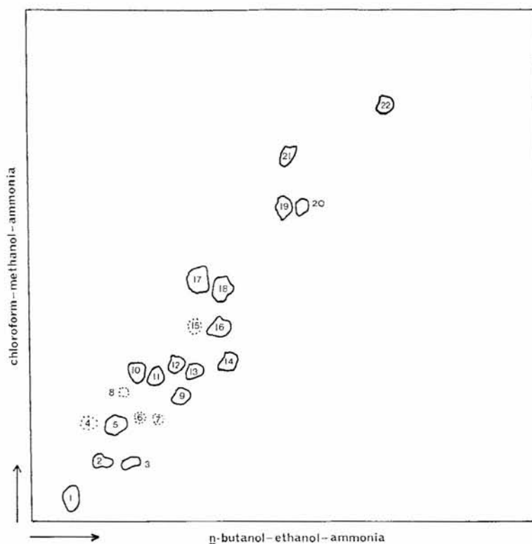
Fig. 1. Separation of tryptophan derivatives in ethanol extract of 7-day old P. aquatica seedlings by two-dimensional TLC. The identification of the numbered spots is indicated; the colour given by Van Urk-Salkowski reagent is shown in brackets as a colour region, colour name and page number from the Horticultural Colour Chart 7 . Only the colour for compounds not included by Ehmann 4 is given. 1 = Tryptophan, 5-methoxytryptophan; 2 = 5-hydroxy-N-methyltryptamine (blue, Sea Blue, 119); 3 = 5-hydroxytryptamine; 4 = unknown (blue, Princes Blue, 98); 5 = 3-methylaminomethylindole (violet, Campanula Violet, 37); 6 = unknown (red, Rose Madder, 23); 7 = unknown (yellow, Majolica Yellow, 102); 8 = unknown (blue, Princes Blue, 98); 9 = 3-aminomethylindole (violet, Campanula Violet, 37); 10 = 5-methoxy-N-methyltryptamine (blue, Princes Blue, 98); 11 = N-methyltryptamine (blue, Princes Blue, 98); 12 = 5-methoxytryptamine; 13 = tryptamine; 14 = 5-hydroxy-N,N-dimethyltryptamine; 15 = unknown (mauve, Dauphin's Violet, 117); 16 = gramine; 17 = unknown (yellow-grey, Yellow Ochre, 101); 18 = unknown (blue-grey, Wisteria Blue, 154); 19 = 5-methoxy-N,N-dimethyltryptamine (blue, Cornflower Blue 164); 20 = N,N-dimethyltryptamine (blue, Princes Blue, 98); 21 = unknown (purple, Magnolia Purple, 114); 22 = indole-3-aldehyde.
