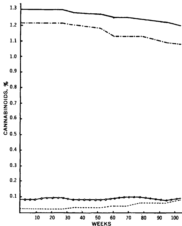
Figure 1— C. sativa L. plant material stored at -18^{\circ} . Key: —, (-) - \Delta^9 -trans-tetrahydrocannabinol; ---, (-) - \Delta^9 -trans-tetrahydrocannabinolic acid; \circ —, cannabidiol; and \square —, cannabinol.
