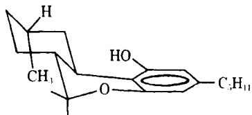
XV: C-9 axial hexahydrocannabinol
