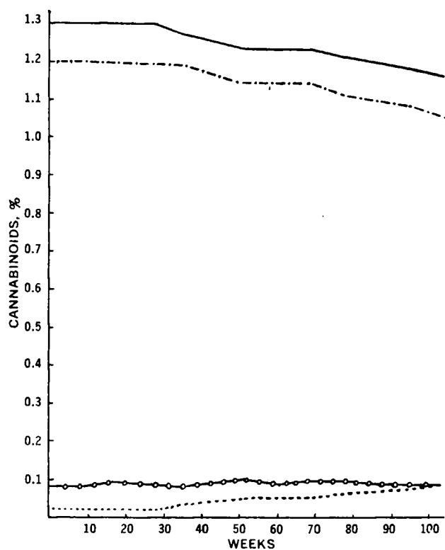
Figure 2— C. sativa L. plant material stored at 4^{\circ} . Key: —, (-) - \Delta^9 -trans-tetrahydrocannabinol; ---, (-) - \Delta^9 -trans-tetrahydrocannabinolic acid; \circ —, cannabidiol; and \square —, cannabinol.
