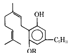
III: cannabigerol monomethyl ether, R = CH 3
