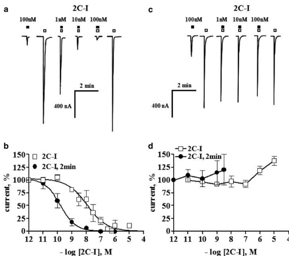
Figure 2 Selective 5-HT 2A receptor antagonism by 2C-I (2,5-dimethoxy-4-iodo-phenyl)ethylamine. (a) Representative tracing illustrates the blockade of the 100 nM 5-HT-evoked current by coapplication of 1, 10 or 100 nM 2C-I to a single oocyte expressing 5-HT 2A receptors. Solid squares represent 2C-I applications, open squares depict 100 nM 5-HT additions. Note that 100 nM 2C-I alone caused a small reproducible current, consistent with its partial agonism. (b) The coapplication of different concentrations of 2C-I plus 100 nM 5-HT blocked the 5-HT-induced currents in a concentration-dependent manner at the 5-HT 2A receptor (open squares). A 2-min preapplication of 2C-I increased the magnitude of the blockade about 100-fold (solid circles). (c) Representative polygraph recording shows, in the same oocyte, that 2C-I did not significantly reduce the 10 nM 5-HT-evoked currents at the 5-HT 2C receptor. Solid squares represent the 2C-I applications; open squares depict 10 nM 5-HT additions. Consonant with its partial agonist profile, 100 nM 2C-I per se caused a current amounting to 35% of the 10 nM 5-HT response. (d) 2C-I did not block the 10 nM 5-HT-induced currents in an oocyte expressing 5-HT 2C receptors when 2C-I was either coapplied or preapplied for 2 min. Coapplications of 2C-I larger than 3 nM were not tested in view of its partial agonism. Symbols indicate the mean average normalized current, and bars the s.e.m. At least four separate oocytes from two batches of oocytes were analyzed per protocol in all panels.
