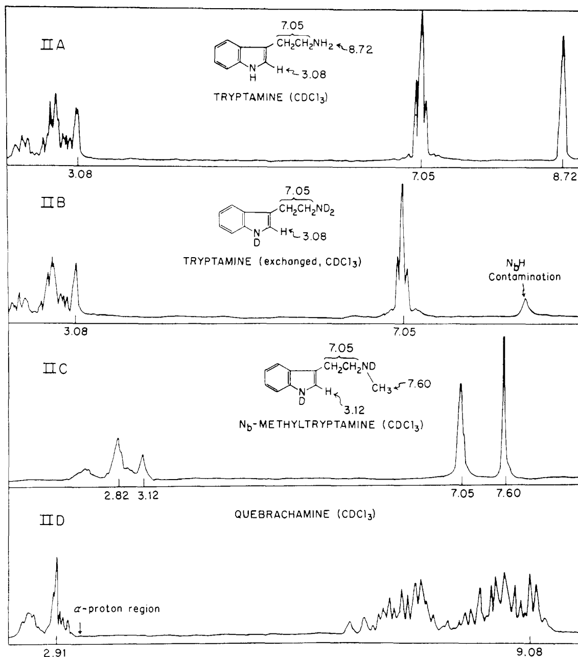
Fig. 2.—Values in \tau .
