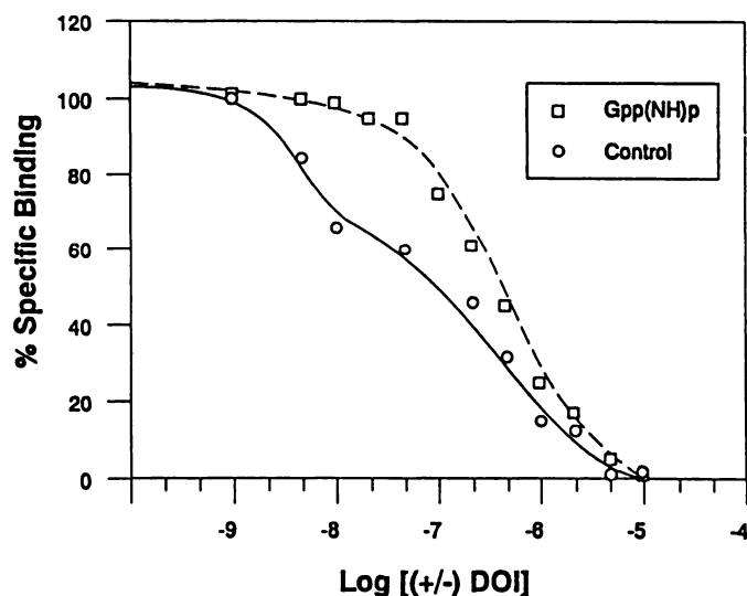
Fig. 1. Effect of Gpp(NH)p on DOI competition for [ 3 H]ketanserin binding to the cloned human 5-HT 2 receptor expressed in L-M(TK - ) cells. Before the addition of 100 \mu M Gpp(NH)p, the competition curve for DOI is biphasic. After addition, the slope of the competition curve is shifted to a lower affinity but steepened, consistent with a single population of noninteracting sites.
