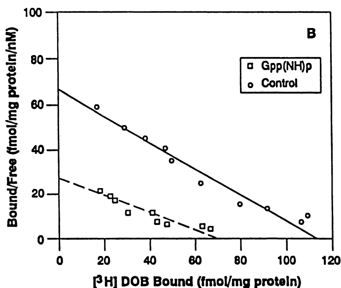
Fig. 2. Scatchard analyses of the binding of [ 3 H]ketanserin (A) and [ 3 H]DOB (B) to the cloned human 5-HT 2 receptor expressed in L-M(TK - ) cells. For each radioligand, full saturation curves were run in the presence and absence of 100 \mu M Gpp(NH)p as paired controls. Mianserin (1 \mu M) was used to define nonspecific binding. All data points were run in triplicate.
