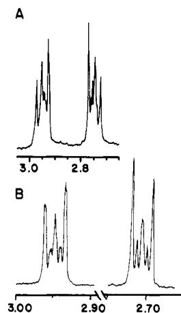
Figure 1. (A) The 360-MHz spectrum for the \alpha ( \text{H}_a and \text{H}_{a'} ) and \beta ( \text{H}_b and \text{H}_{b'} ) protons of bufotenin free base in \text{CDCl}_3 . (B) The 360-MHz spectrum for the \alpha and \beta protons of psilocin free base in \text{CDCl}_3 . The chemical shifts are measured relative to an internal \text{Me}_4\text{Si} standard.
