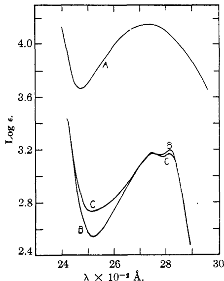
Fig. 1.—A, Synthetic tetrahydrocannabinol in ether. Ghosh, Todd and Wilkinson, J. Chem. Soc. , 1121 (1940), report \log \epsilon = 4.046 at 2755 \text{ \AA} . in ethanol. B, Tetrahydrocannabinol prepared by isomerization of cannabidiol. The spectra of the low- and high-rotating forms were so nearly identical that they are shown here as one curve. C, Cannabidiol.
