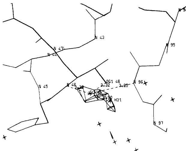
Figure 7. Another carboxy-binding region is indicated by these -4.5 kcal/mol contours near the amino termini of helices \alpha\text{C} and \alpha\text{F} of dihydrofolate reductase. 22 Such regions have been discussed by Hol et al. 28 See text. A chloride ion (Cl H2) has been observed 22 at this site, as shown.
