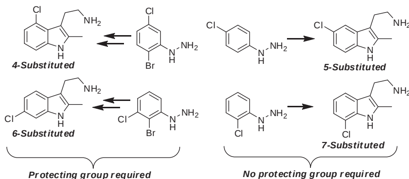
Scheme 1. The traditional syntheses of 4- and 6-chloro-2-methyl-3-aminoethylindole syntheses via Fischer indolization are poorly regioselective. Using bromine as a protecting group to block reactivity on the aromatic ring, followed by debromination, can overcome this limitation.
