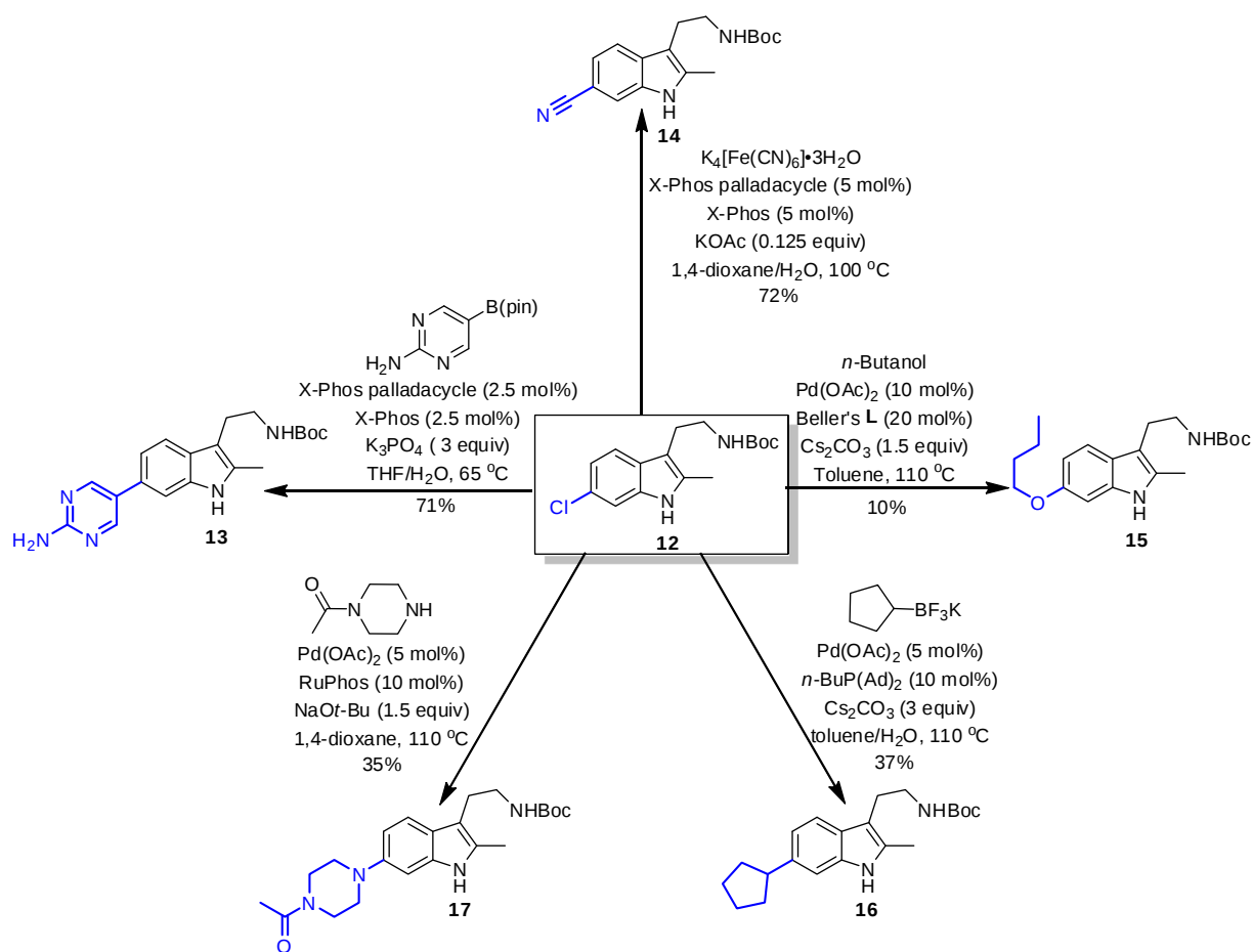
Scheme 5. Late-stage diversification of 6-chloro-2-methyl-3-aminoethylindole.
