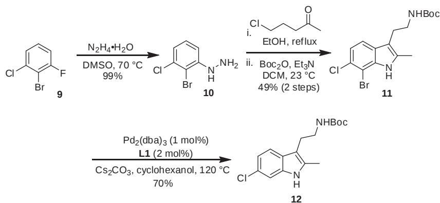
Scheme 4. Synthesis of Boc-protected 6-chloro-2-methyl-3-aminoethylindole 12 .
