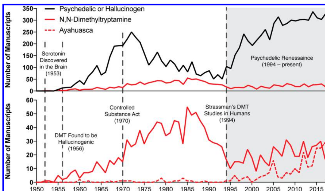
Figure 5. Timeline of important events related to research on DMT and other psychedelics. Note the different y-axis scales for the two graphs. Data related to DMT are presented on both graphs. The data presented here were obtained from Scifinder (Chemical Abstracts Service: Columbus, OH, 2017; accessed Nov 20, 2017) using the search terms “psychedelic or hallucinogen,” “N,N-dimethyltryptamine,” and “ayahuasca”.
