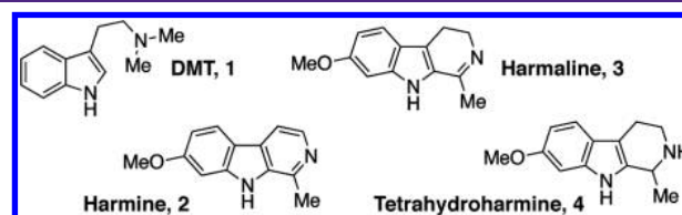
Figure 1. Chemical structures of the key psychoactive alkaloids found in ayahuasca.
