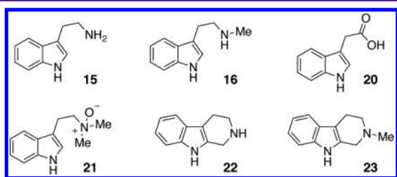
Figure 4. Metabolites of DMT produced from rat brain homogenates.
