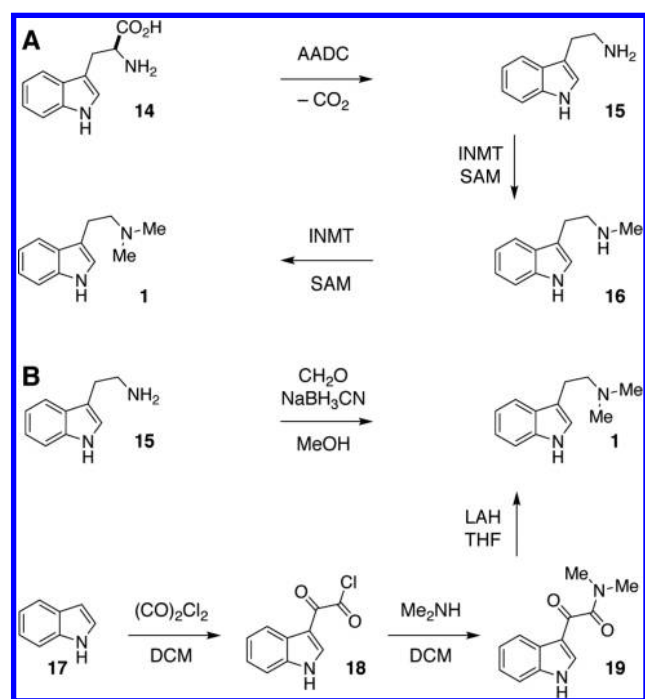
Figure 3. Synthesis of DMT. (A) Biosynthesis of DMT. (B) Chemical syntheses of DMT.
