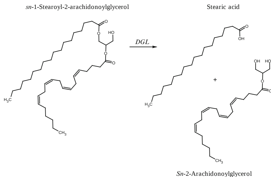
Fig. 2 Reaction scheme for diacylglycerol lipase action. Membrane-associated diacylglycerol, shown here as 1-stearoyl-2-arachidonoylglycerol, is hydrolysed to generate free fatty acid and 2-acylglycerol, both of which are much more water soluble than the parent and may have multiple cellular actions
