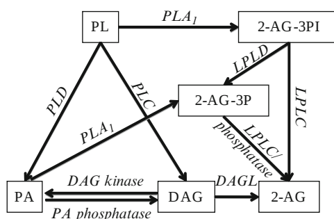
Fig. 3 Alternative routes of 2AG formation. Aside from the canonical route of 2AG formation through PLC/DGL action, diacylglycerol can also be formed via phosphatidic acid generated by PLD action. Additionally, PLA 1 activity can generate a lysophospholipid, which may be used to generate 2AG directly through a LPLC activity, or indirectly through a LPLD/LPLC sequence. Phospholipase A 1 hydrolysis of phosphatidic acid can also allow generation of 2AG, through the intermediate 2AG-3-phosphate, which can then be hydrolysed by a phosphatase/lysophospholipase C activity
