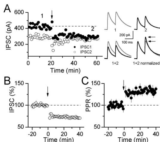
Figure 1. Long-Term Depression at Hippocampal Inhibitory Synapses
