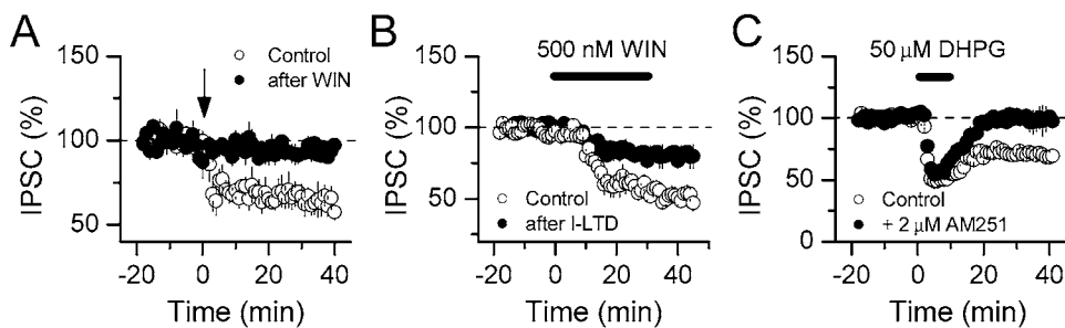
Figure 5. CB 1 Rs Mediate I-LTD- and DHPG-Induced Depression of IPSCs
