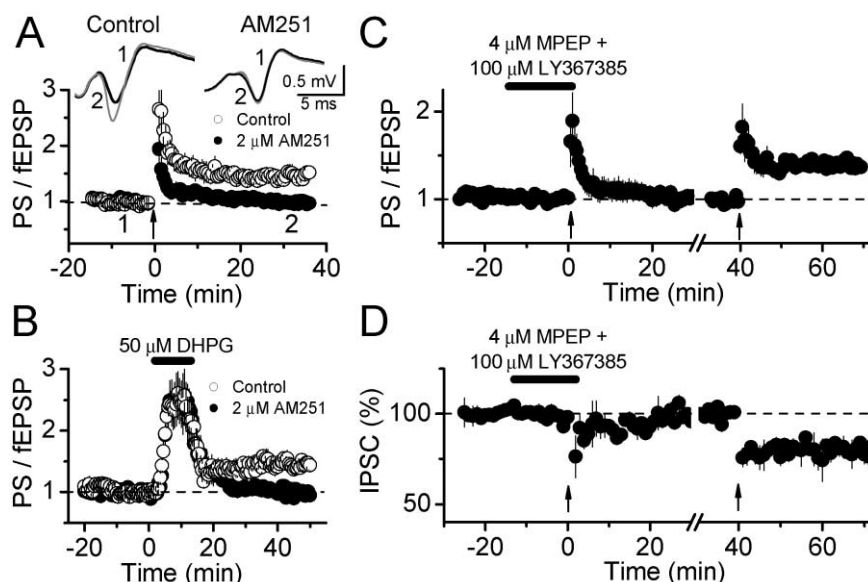
Figure 8. I-LTD Is Involved in E-S Coupling Potentiation
