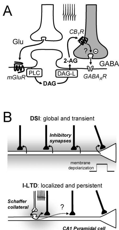
Figure 9. I-LTD: Mechanism of Induction and Functional Properties (A) Glutamate release from Schaffer collaterals as a result of high-frequency stimulation activates postsynaptic mGluR1/5 , leading to PLC activation and DAG formation. DAG is then converted by the DAG lipase (DAG-L) into 2-AG, which inhibits GABA release by acting on presynaptic CB_1Rs . The mechanisms downstream from CB_1R underlying I-LTD are still unknown. (B) Temporal and spatial differences between I-LTD and DSI. While DSI produces a generalized but transient depression of cannabinoid-sensitive GABAergic inputs (in black), I-LTD is more localized and long lasting. DSI is commonly triggered by a brief ( \sim 5 s) postsynaptic depolarization of the CA1 pyramidal cell, whereas I-LTD induction requires glutamate release from Schaffer collaterals and CB_1R activation during several minutes.
