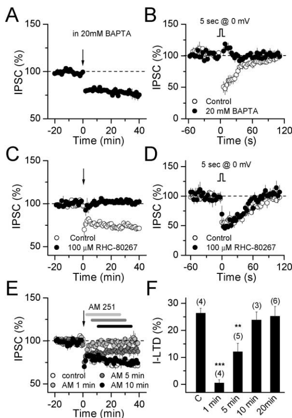
Figure 7. Cannabinoid Release and Duration of CB 1 R Activation Differ between I-LTD and DSI
