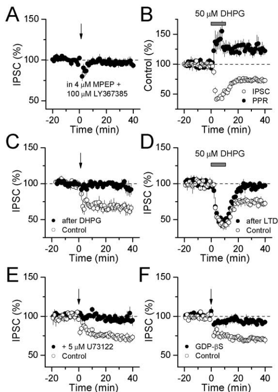
Figure 3. I-LTD Requires Postsynaptic mGluR1/5 Activation
