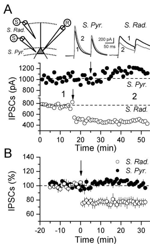
Figure 2. HFS Stimulation in stratum radiatum , but not stratum pyramidale , Induces LTD of Inhibitory Synapses at CA1 Pyramidal Cells
