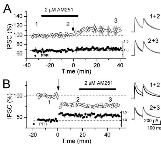
Figure 4. CB 1 Receptors Are Necessary for I-LTD Induction but Not Maintenance
