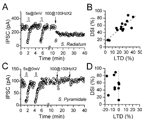
Figure 6. I-LTD versus DSI
