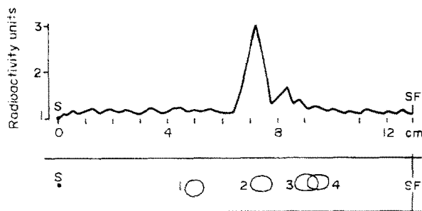
FIG. 5. Thin-layer chromatogram and radioactivity scan of the "neutral fraction" obtained by TLE. Solvent: n -butanol-acetic acid-water (4:1:5). Reference compounds: 1 = mescaline.HCl, 2 = N -acetyl-mescaline, 3 = 3,4,5-TMPAA, 4 = 3,4,5-TMBA. S = origin, SF = solvent front. 200 \mu m silica gel G F254 .
