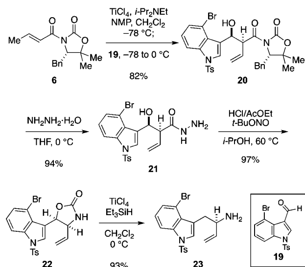
Scheme 4. Synthesis of 23
