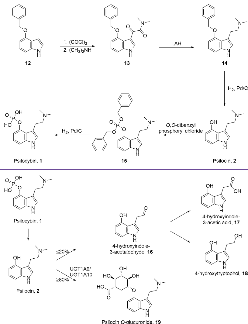
Figure 2. Phase I and phase II metabolites of psilocybin. 19
