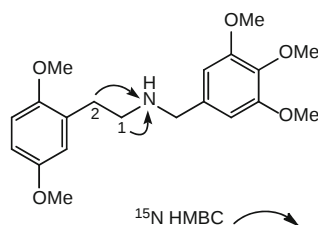
(g) Compound (5)
