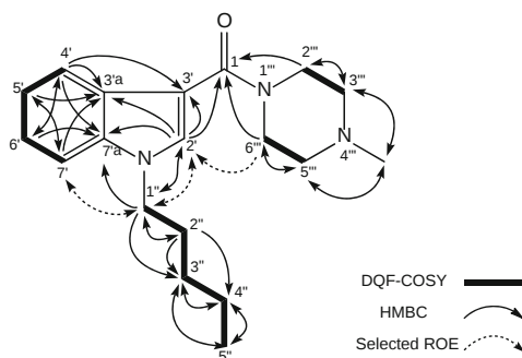
(e) Compound (4)
