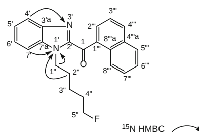
(b) Compound (1)
