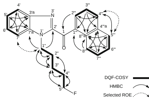
(c) Compound (2)
