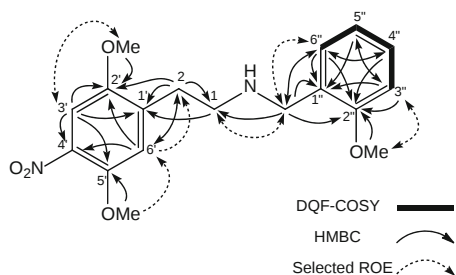
(e) Compound (4)
