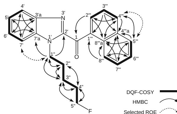
Fig. 3 Double quantum filtered correlation spectroscopy (DQF-COSY), selected heteronuclear multiple-bond correlation (HMBC), and selected rotating frame nuclear Overhauser effect (ROE) correlations for compounds 1 (a), 2 (c), 4 (e) and 5 (f), and ^{15}\text{N} HMBC correlations for compounds 1 (b), 2 (d), and 5 (g)
