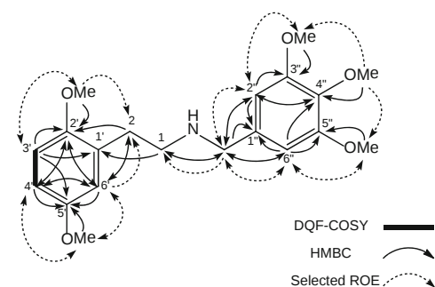
Fig. 3 Double quantum filtered correlation spectroscopy (DQF-COSY), selected heteronuclear multiple-bond correlation (HMBC), and selected rotating-frame nuclear Overhauser effect (ROE)
