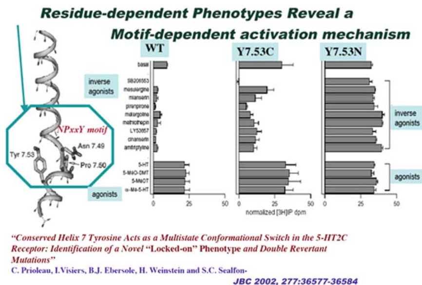
Fig. 17.1 Data illustrating the functional role of Y7.53 in the NPxxY motif: Different activated states of the 5-HT 2C receptors are produced by mutations at the 7.53 locus. The Y7.53C mutation produces a canonical constitutively activated phenotype, characterized by increased basal activity compared with WT, reduction of the basal activity by various inverse agonists, and activation by various agonists. In contrast, the constitutive activity of the Y7.53N mutant is shown to be irreversible (by any of the inverse agonists), and various agonists are unable to activate further the receptor, which appears locked in an “on” state.
