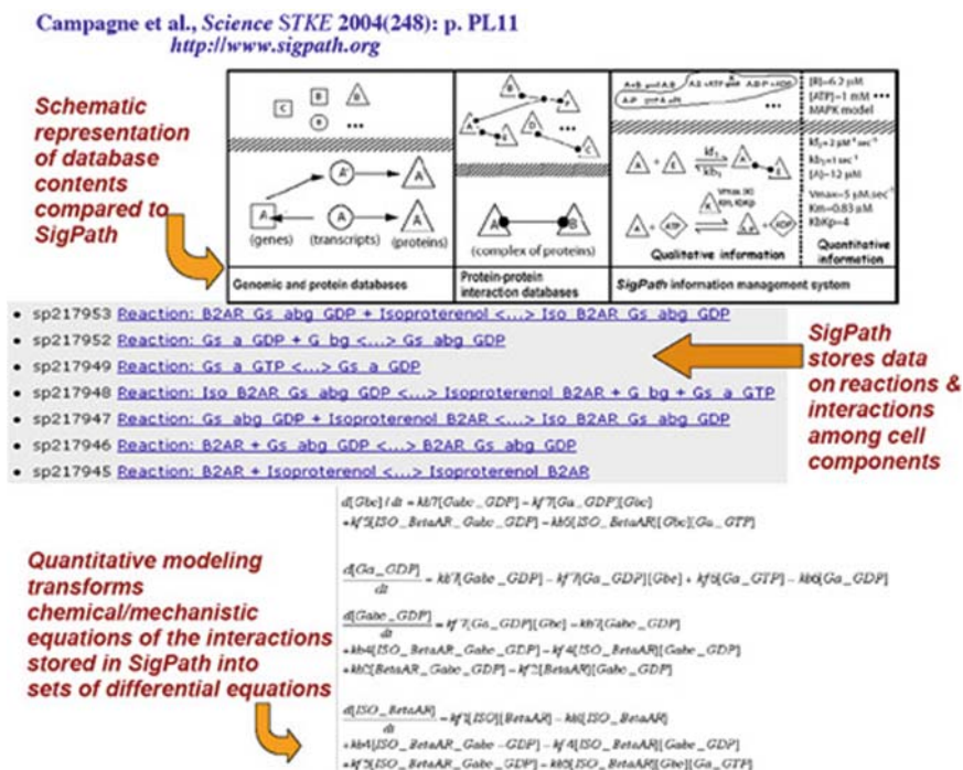
Fig. 17.4 Schematic representations of SigPath 15 characteristics: SigPath contents compared with traditional databases show the information management characteristics that include detailed reactions among the entries, as well as their quantitative parameters; the stored reaction information is illustrated, with specific identification numbers (sp-id of the form spxxxx, where x are running numbers) assigned by SigPath; the transformation of the reaction information into ODEs performed through transparent connections to mathematical modeling environments such as VirtualCell. 12
