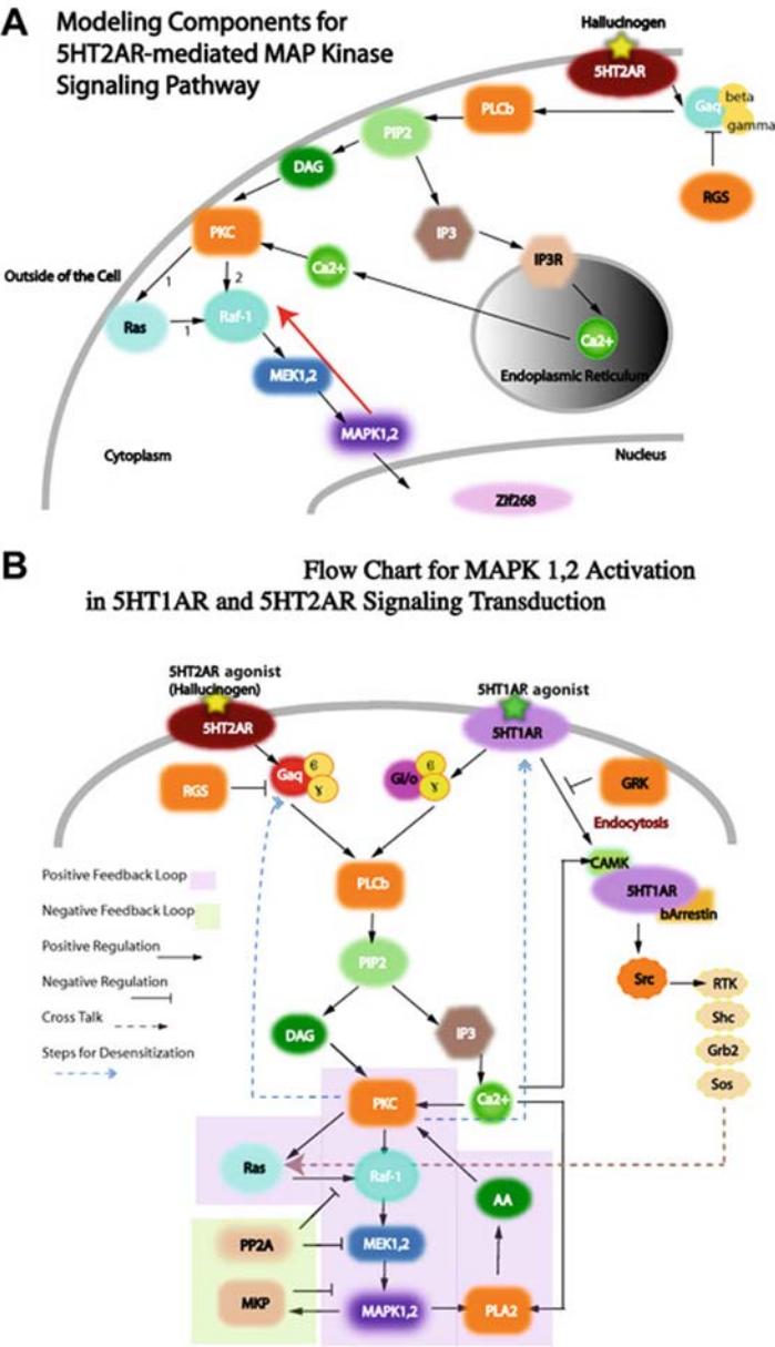
Fig. 17.5 Schematic representations of signaling pathways from 5-HT receptors to the MAPK system. (A) Signaling pathway triggered by activation of the 5-HT2A receptor coupled to G \alpha_q ; and (B) A putative combination of signaling pathways activated by ligand binding to both 5-HT2A and 5-HT1A receptors.
