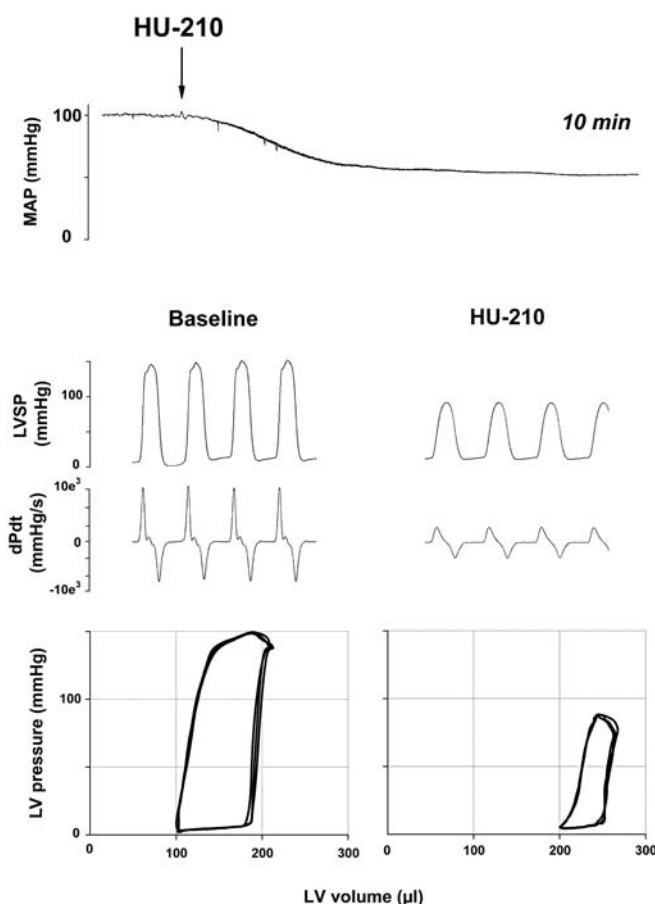
Fig. 2. Hemodynamic effects of HU-210 in anesthetized rat. Representative recordings of the effects of HU-210 (30 \mu\text{g/kg} i.v.) on mean arterial pressure (MAP, top panel), cardiac contractility (LVSP and dP/dt ; middle panel), and pressure-volume (PV) relations (bottom panel) in a pentobarbital-anesthetized rat. The arrow indicates the injection of the drug. The decrease of the amplitude of PV loops and their shift to the right are indicative of decreased cardiac contractile performance
