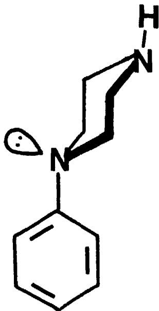
FIG. 2. Structure of 1-PP in a conformationally reasonable form.
