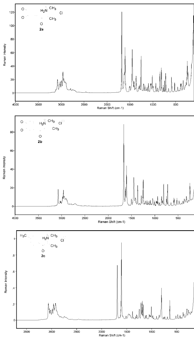
Figure 5 - FT-Raman spectra of methcathinone analogs 2a-c hydrochloride.
