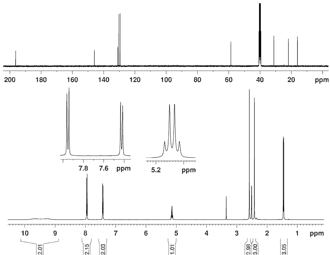
Figure 10 - ^1\text{H} and ^{13}\text{C} NMR data for 2c hydrochloride in DMSO- d_6 .
