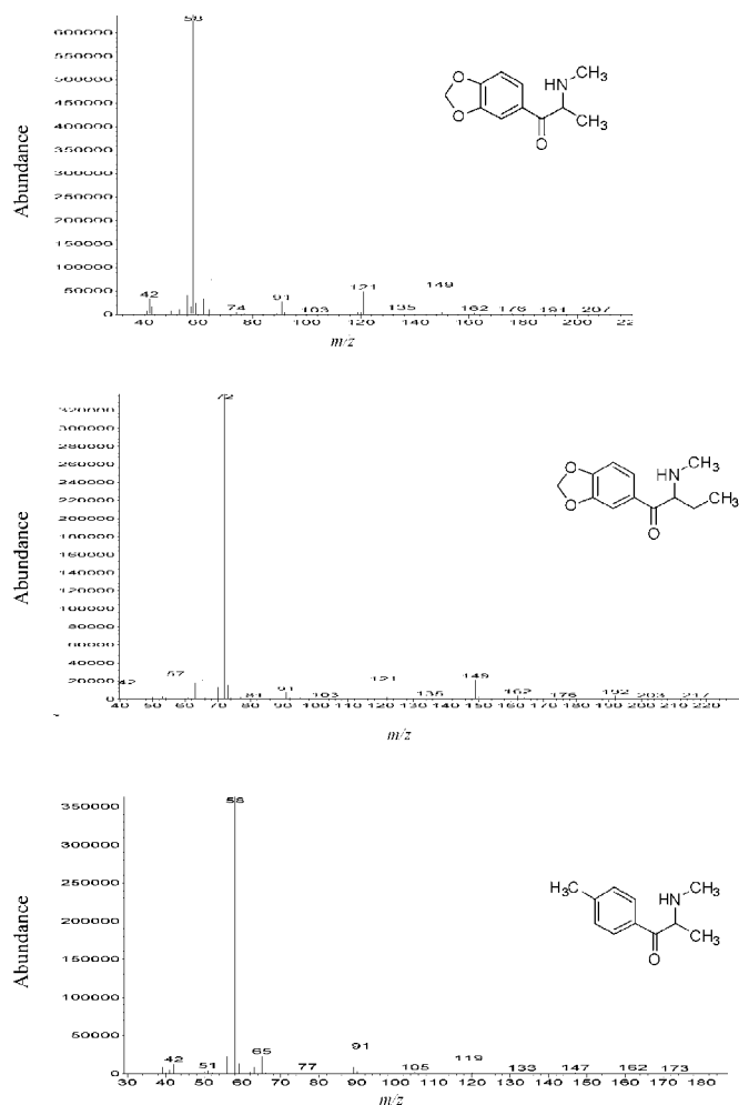
Figure 6 - GC/MS data for analogs 2a (top), 2b (middle), and 2c (bottom).
