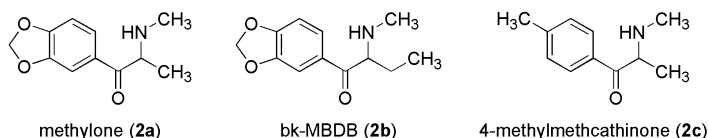
Figure 2 - Structures of methcathinone analogs prepared in this study.
