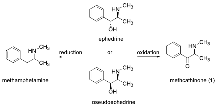
Figure 1 - Ephedrine (or pseudoephedrine) undergoes reduction to give methamphetamine and oxidation to afford methcathinone.
