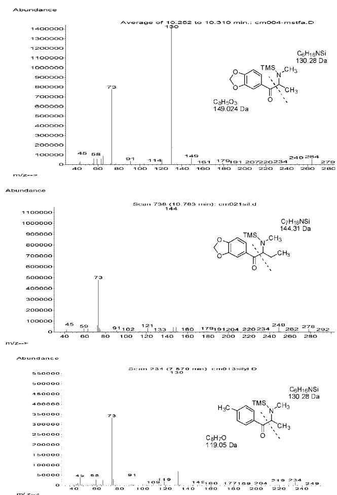
Figure 7 - GC/MS data for trimethylsilylated derivatives 2a (top), 2b (middle), and 2c (bottom).
