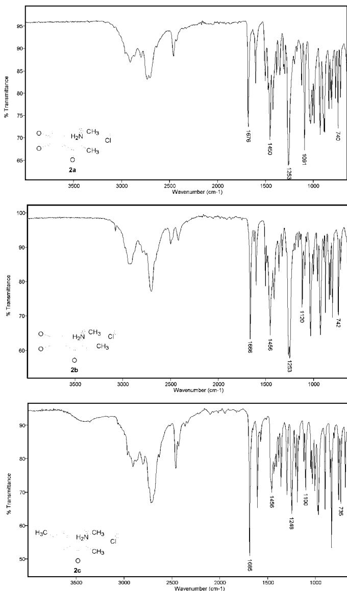
Figure 4 - ATR-FTIR spectra of methcathinone analogs 2a-c hydrochloride.
