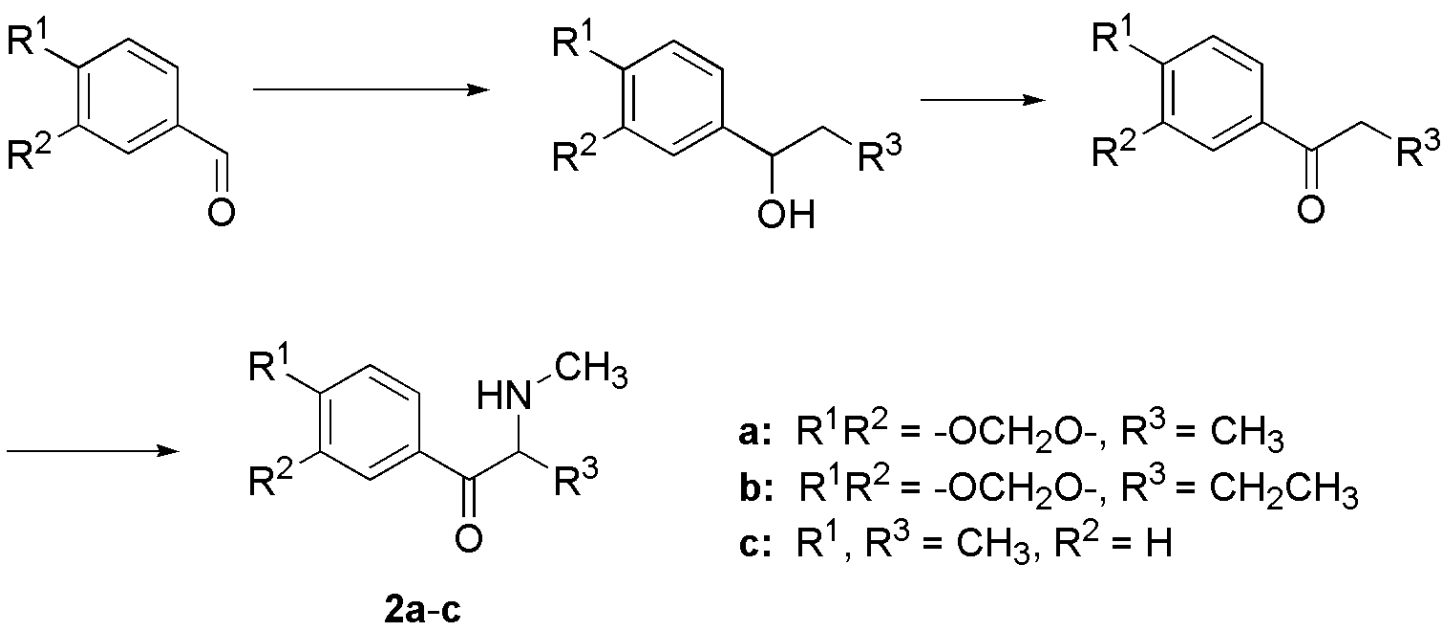
Scheme 1 - Synthetic pathway used for the preparation of methcathinone analogs 2a-c .
