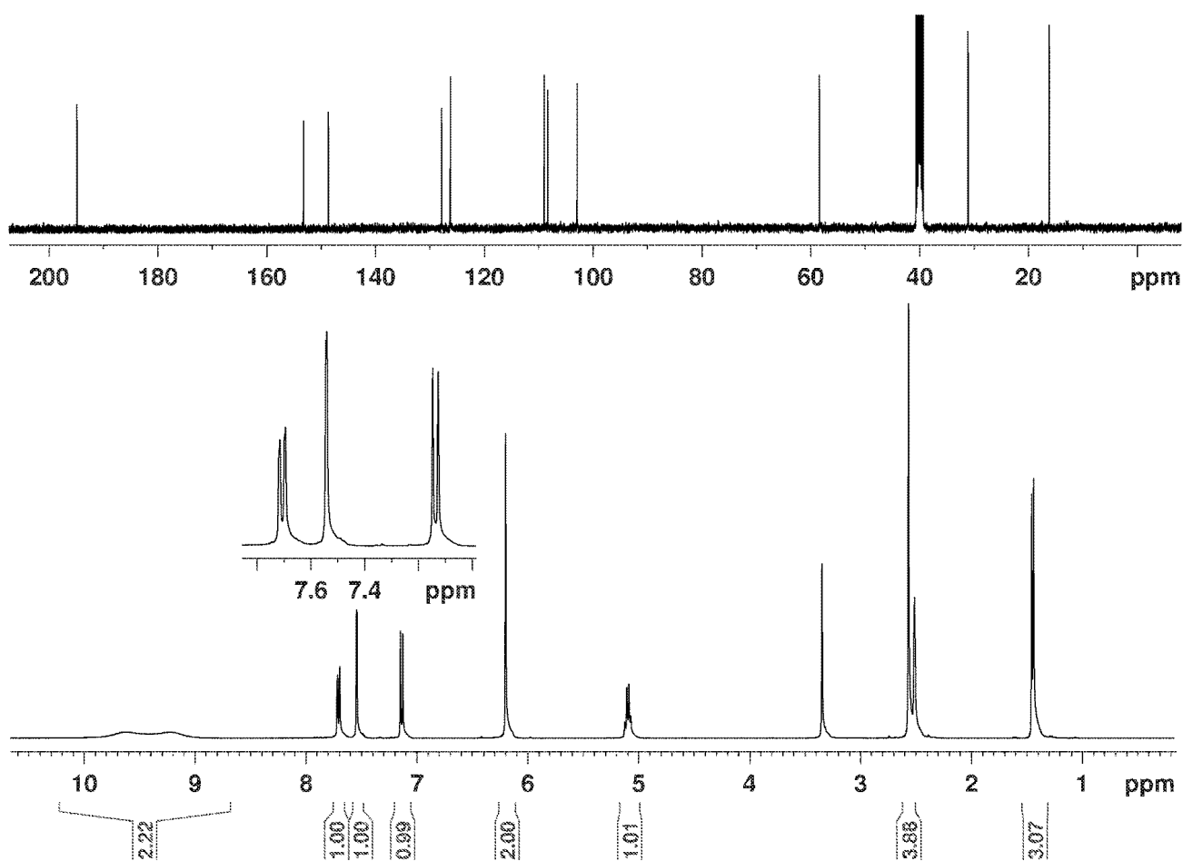
Figure 8 - ^1\text{H} and ^{13}\text{C} NMR data for 2a hydrochloride in DMSO- d_6 .
