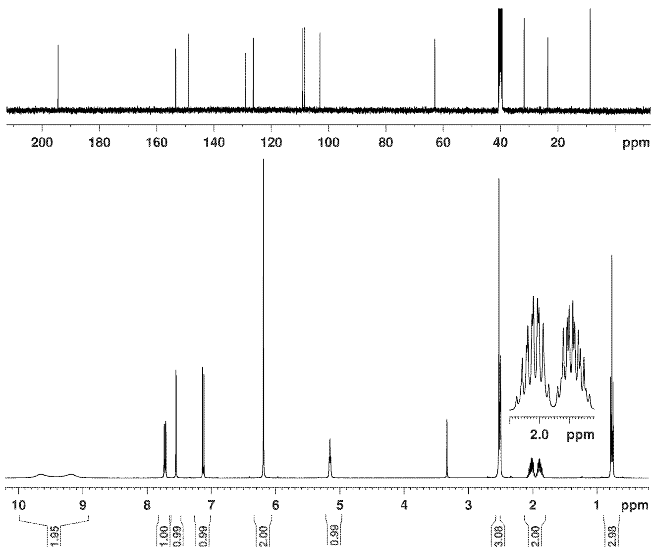
Figure 9 - ^1\text{H} and ^{13}\text{C} NMR data for 2b hydrochloride in \text{DMSO-d}_6 .
