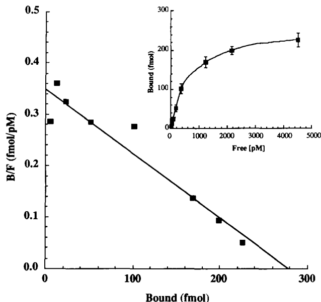
FIG. 5. Binding of ^3\text{H} -11-OH- \Delta^9 -THC-DMH to whole brain P_2 membranes.
