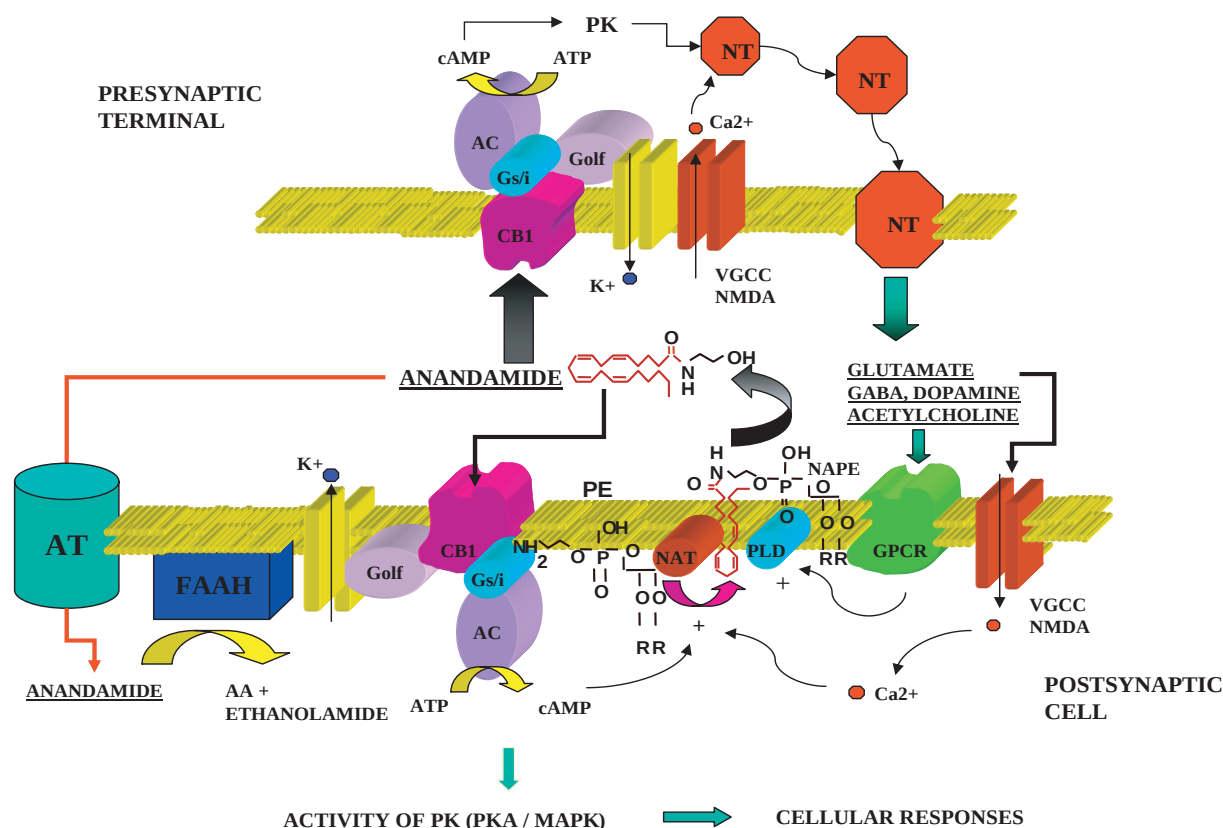
Fig. 2. Overview of the biochemical pathways for synthesis, degradation and cellular actions of the endogenous cannabinoid anandamide. Anandamide is released from a membrane lipid precursor ( N -arachidonoyl-phosphatidylethanolamine, NAPE) by the action of a specific phospholipase D (PLD) activated by depolarization or G-protein-coupled receptor (GPCR) stimulation. NAPE biosynthesis is catalysed by a membrane enzyme, N -acyltransferase (NAT) activated by calcium (Ca 2+ ) and cAMP. Anandamide acts as a retrograde messenger at presynaptic cannabinoid receptors (CB 1 ), where it regulates neurotransmitter release (NT) through its second transduction systems [mainly Ca 2+ incorporated through voltage-gated calcium channels (VGCC) or glutamate NMDA ( N -methyl- D -aspartate) receptors]. Anandamide also acts as a neuromodulator of major transmitter systems, including dopamine, at postsynaptic cells, where it regulates excitability and synaptic plasticity through its modulation of potassium (K + ) channels, and the regulation of a broad spectrum of protein kinases (PK) including protein kinase A and mitogen-activated protein kinases (MAPK). Anandamide action is terminated through a two-step process, which includes, first, its cellular uptake through a specific anandamide transporter (AT) and second, degradation by enzymatic cleavage to arachidonic acid (AA) and ethanolamide by the membrane-bound enzyme fatty acid amidohydrolase (FAAH).
